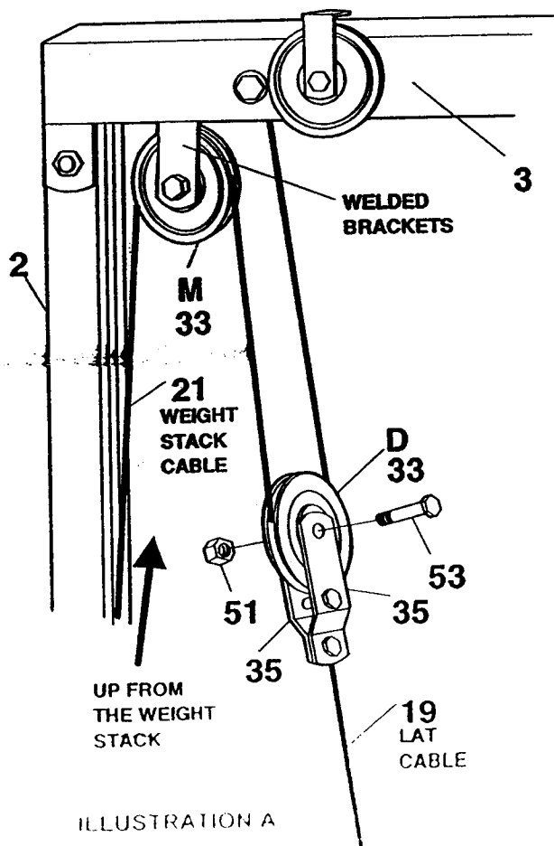
ENTIRE WEIGHT STACK CABLE ROUTING
