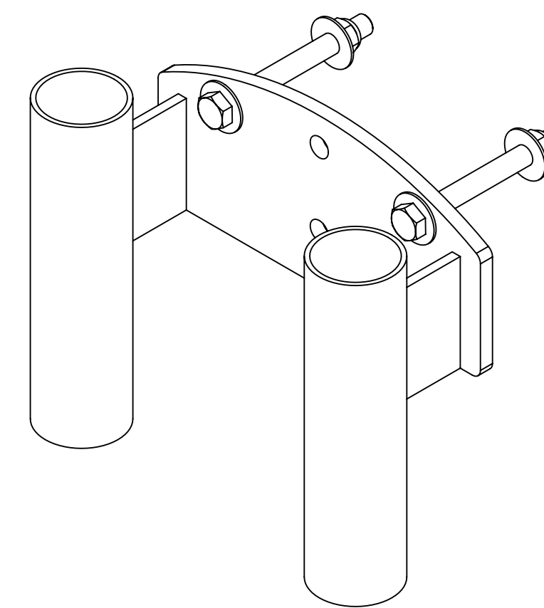
DENALI MOUNTING 2' SUPPORT 6" centers
