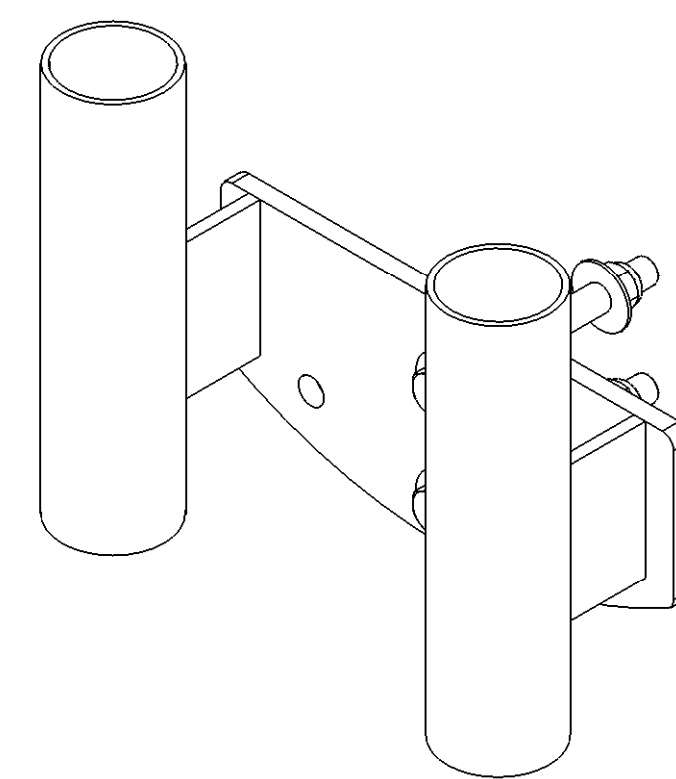
K2 MOUNTING UPRIGHT HOLE PATTERN ( SHOWN EXPLODED)
