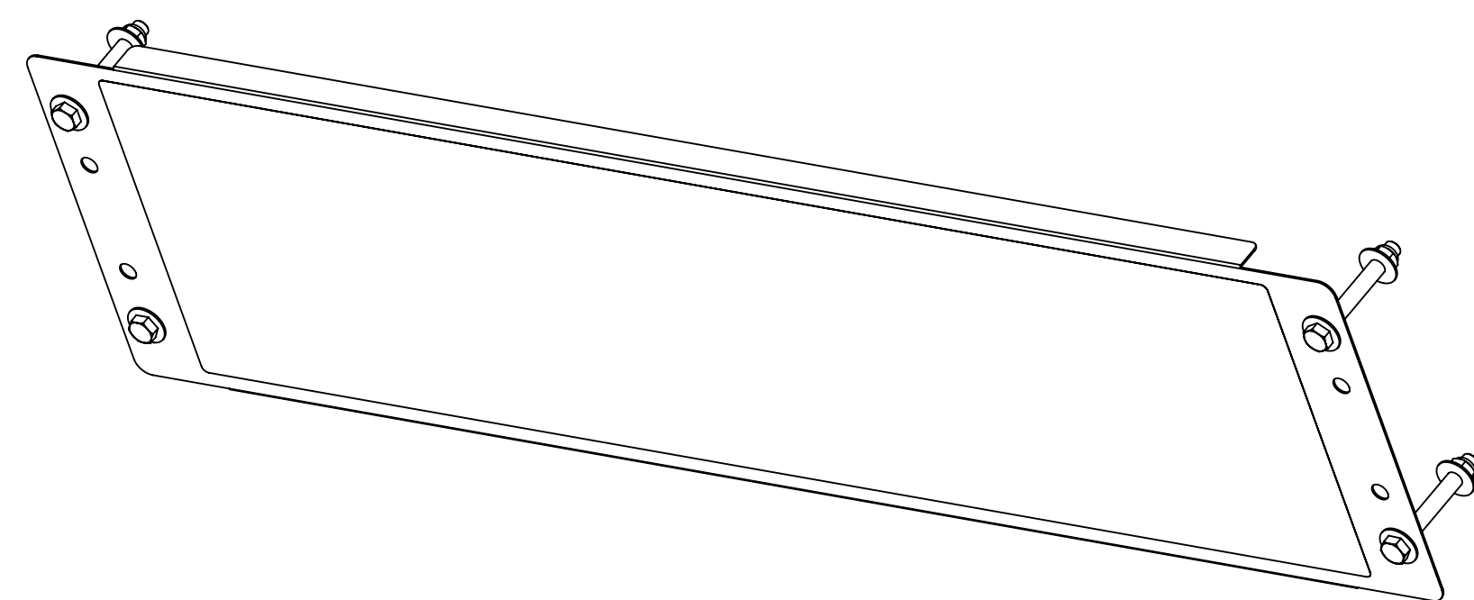
XR25-02 42" NAMEPLATE (SHOWN EXPLODED)
