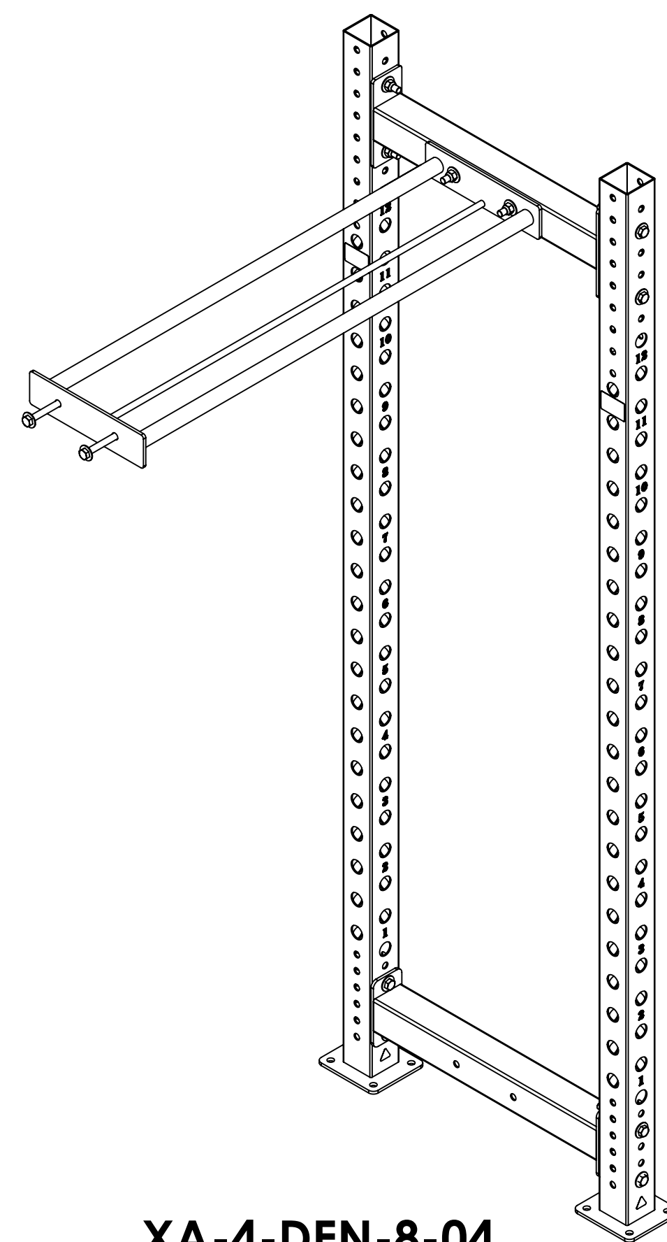
XA-4-DEN-8-04 STORAGE EXTENSION 4' X 2' X 8' (SHOWN EXPLODED)
