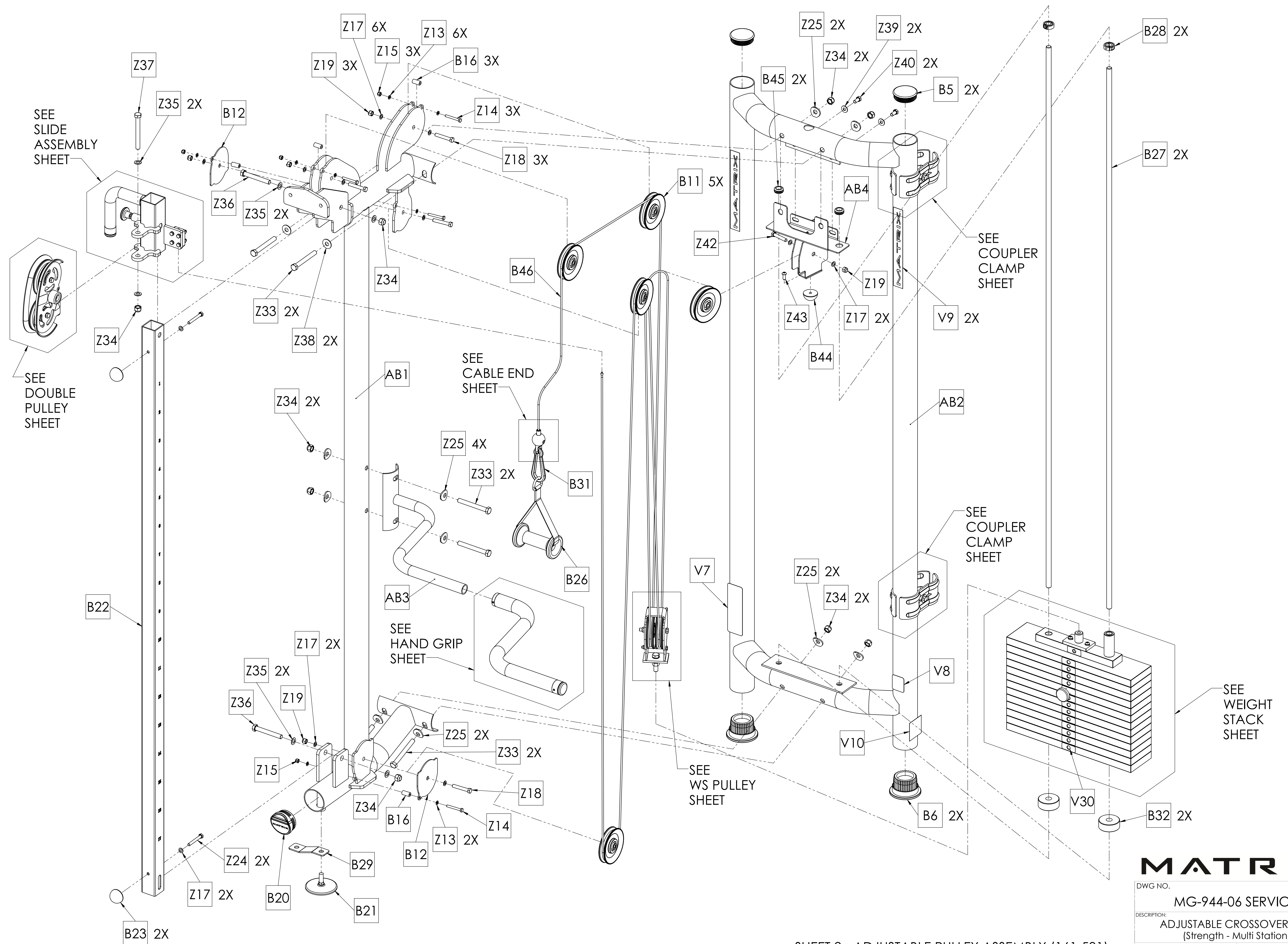
SHEET 2 - ADJUSTABLE PULLEY ASSEMBLY (161-501)
