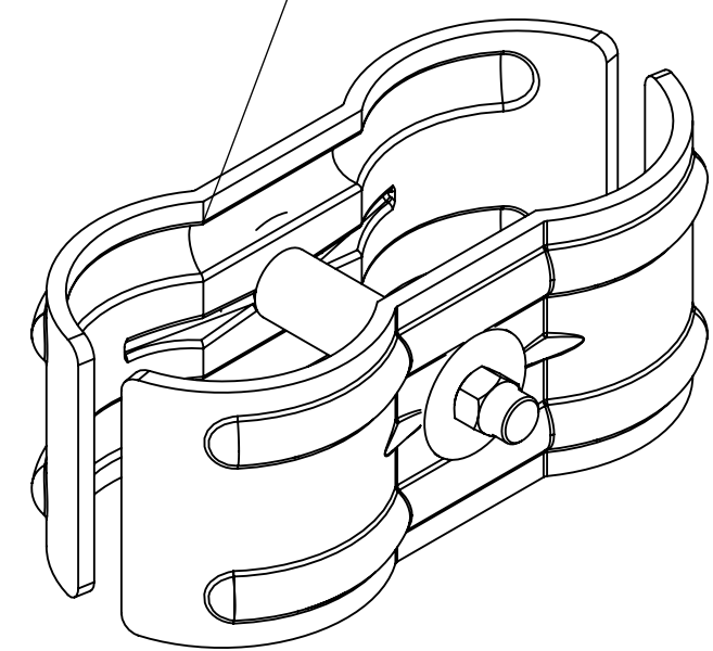
900 SERIES CLAMP (SINGLE)
