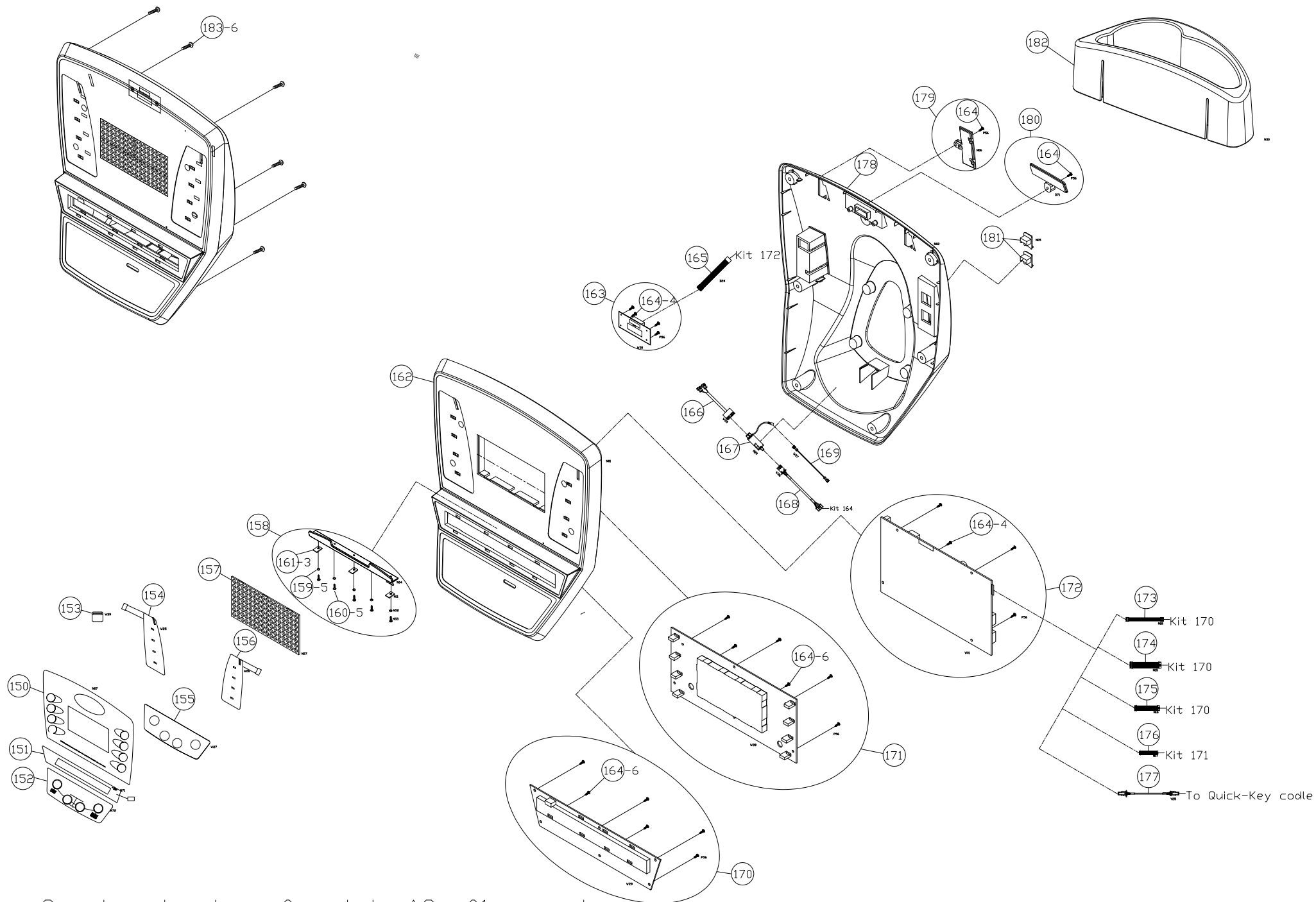
Service drawing of matrix A3x-01 console
