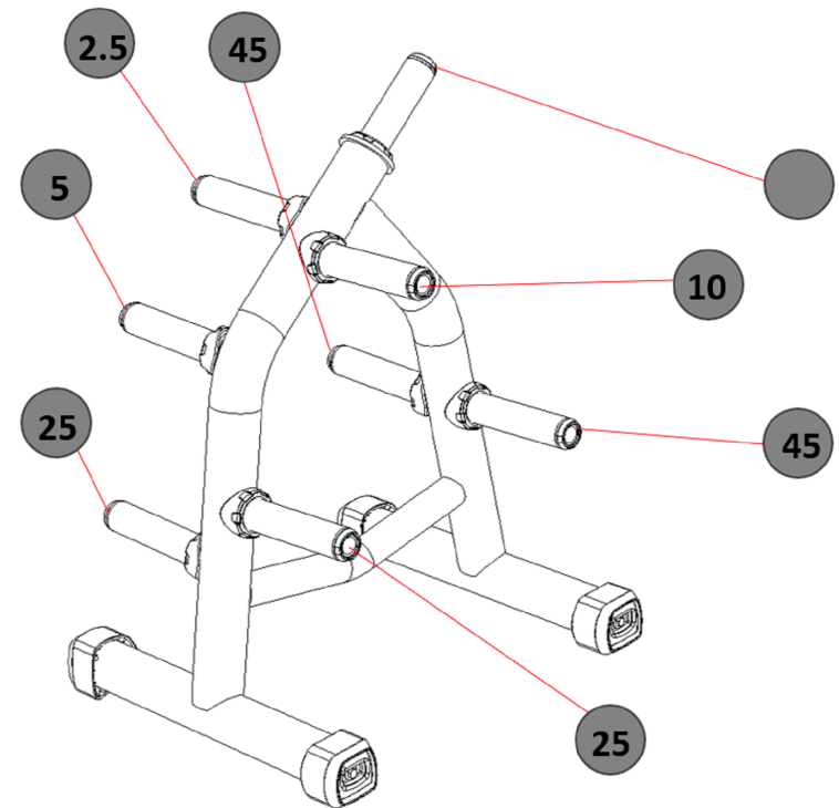
WEIGHT HORN LOCATION DETAIL
