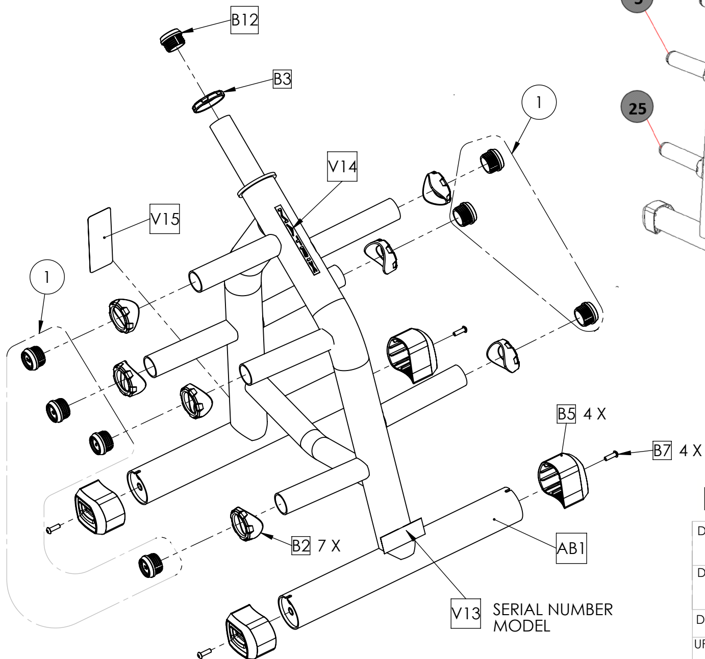
WEIGHT HORN LOCATION DETAIL
