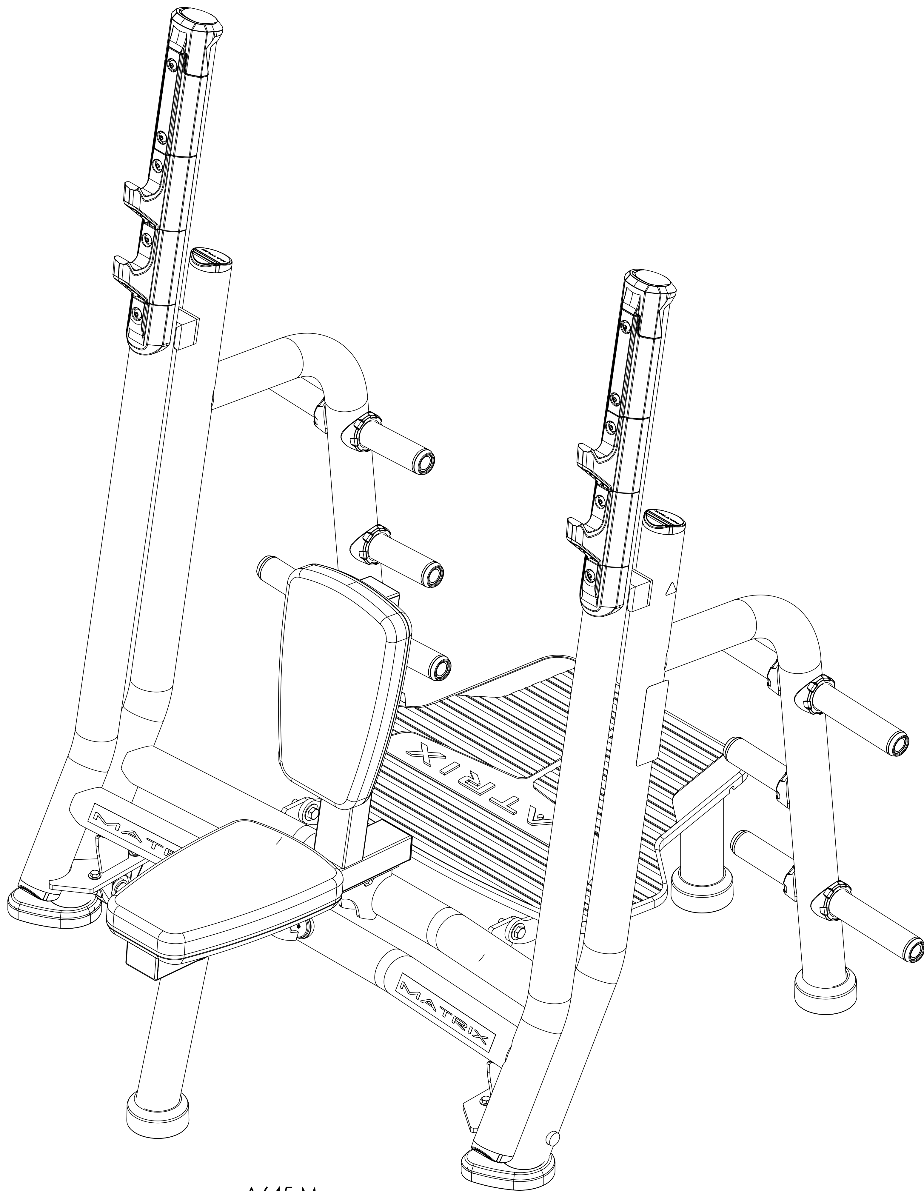
A645 M (SEE SHEET 1 EXPLODED VIEW)
