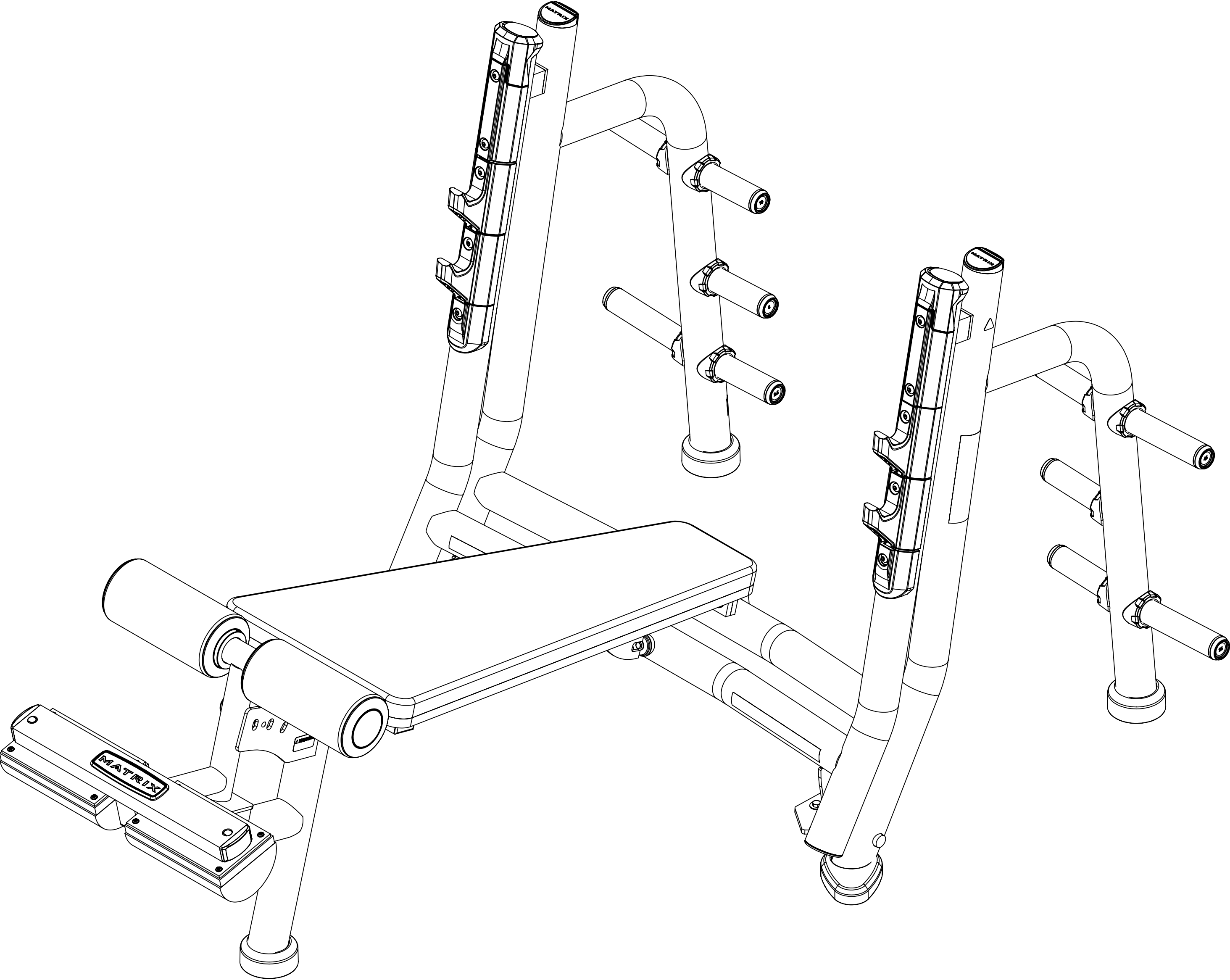
A680 M WITH WEIGHT HORNS SHOWN IN EXPLODED VIEW ( SEE SHEET 1)
