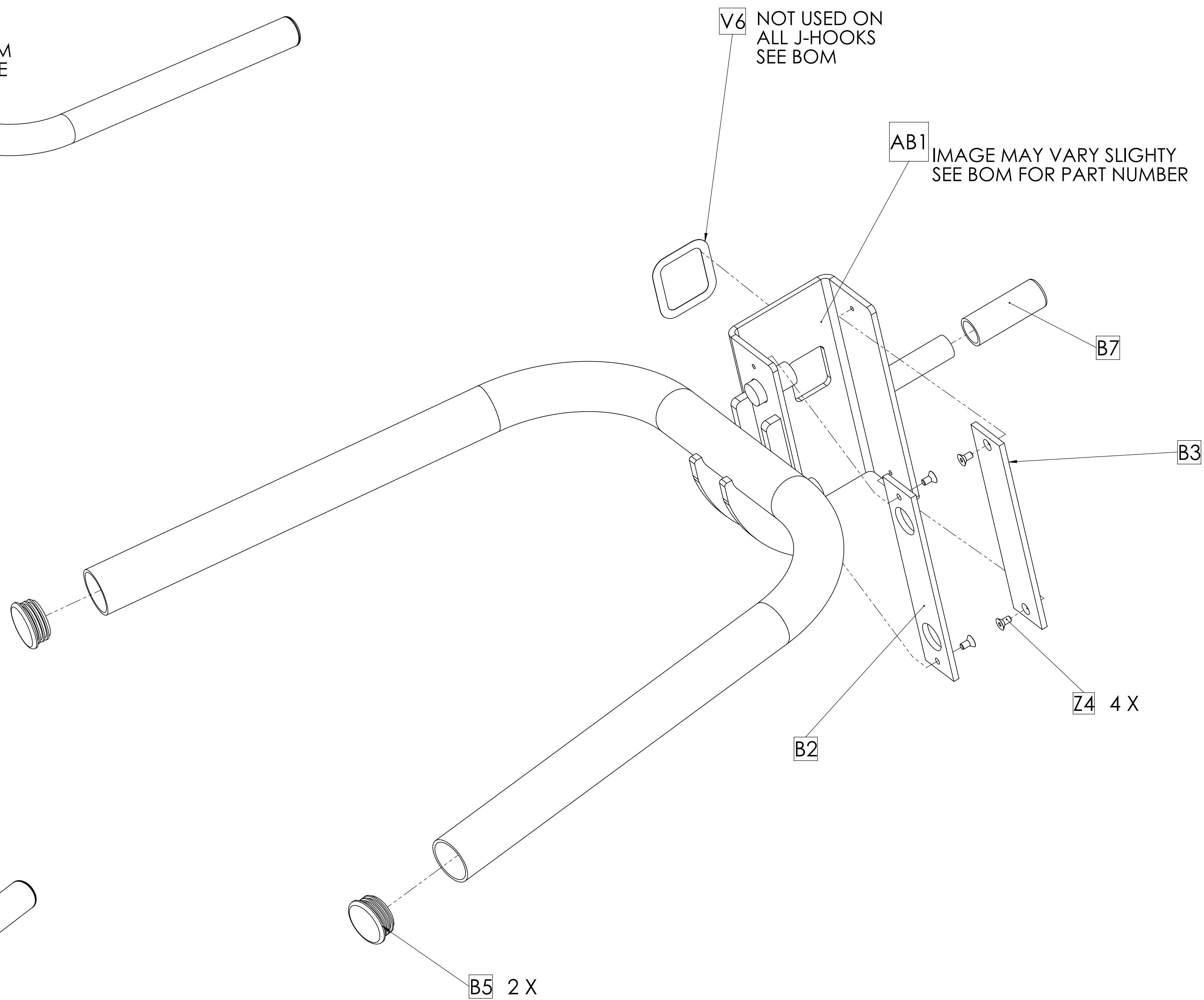
OPT3 M (SHOWN IN EXPLODED VIEW)
