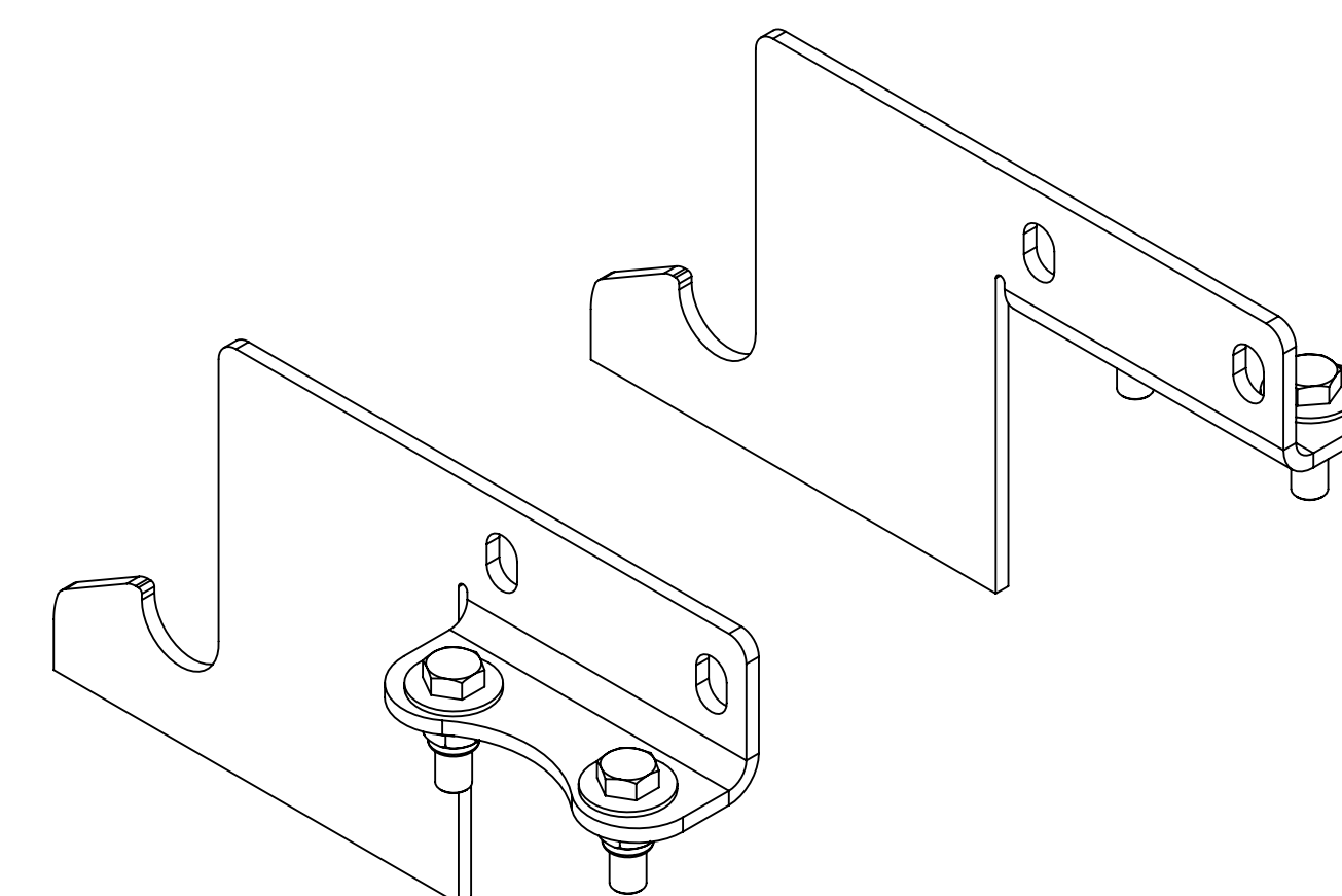
MOPT29 (BRACKET SHOWN FOR REFERENCE)
