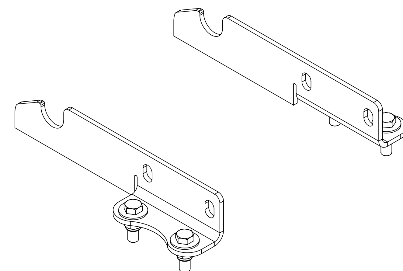
MOPT29P (BRACKET SHOWN FOR REFERENCE)
