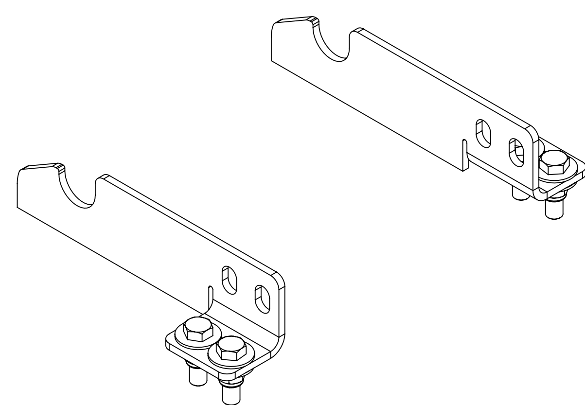
DOPT29P (BRACKET SHOWN FOR REFERENCE)
