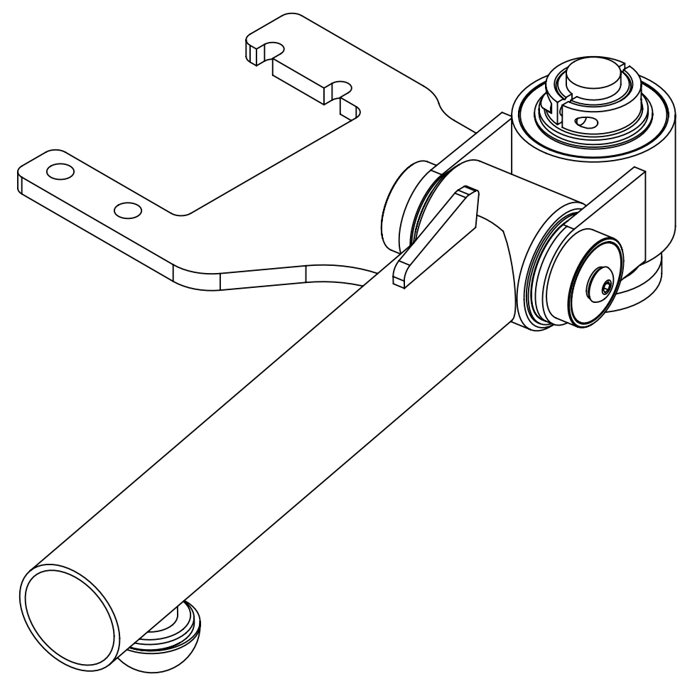
OPT13 (SHOWN IN EXPLODED VIEW)
