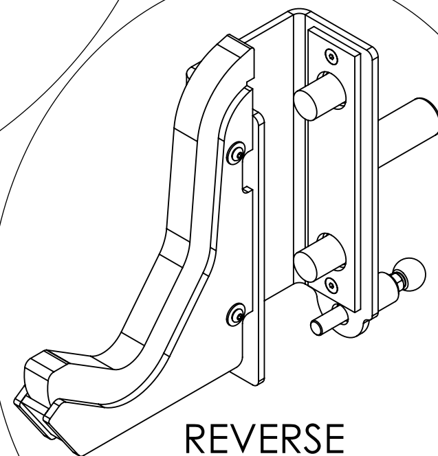
REVERSE LEFT J-HOOK A & MR SERIES
