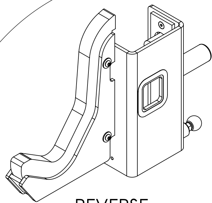
REVERSE LEFT J-HOOK A & MR SERIES
