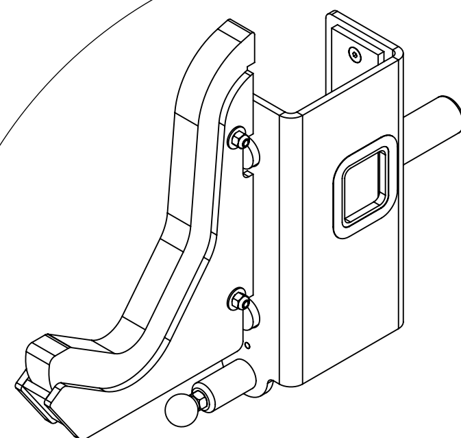
LEFT J-HOOK A & MR SERIES (SHOWN EXPLODED)
