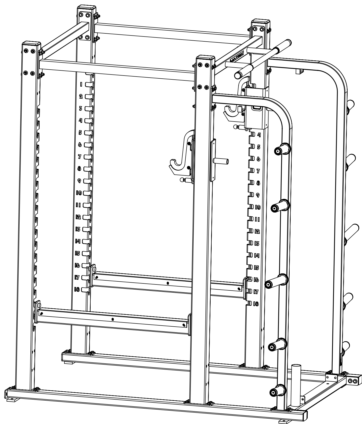
A47-7N-04 WITHOUT SPOTTER STAND
