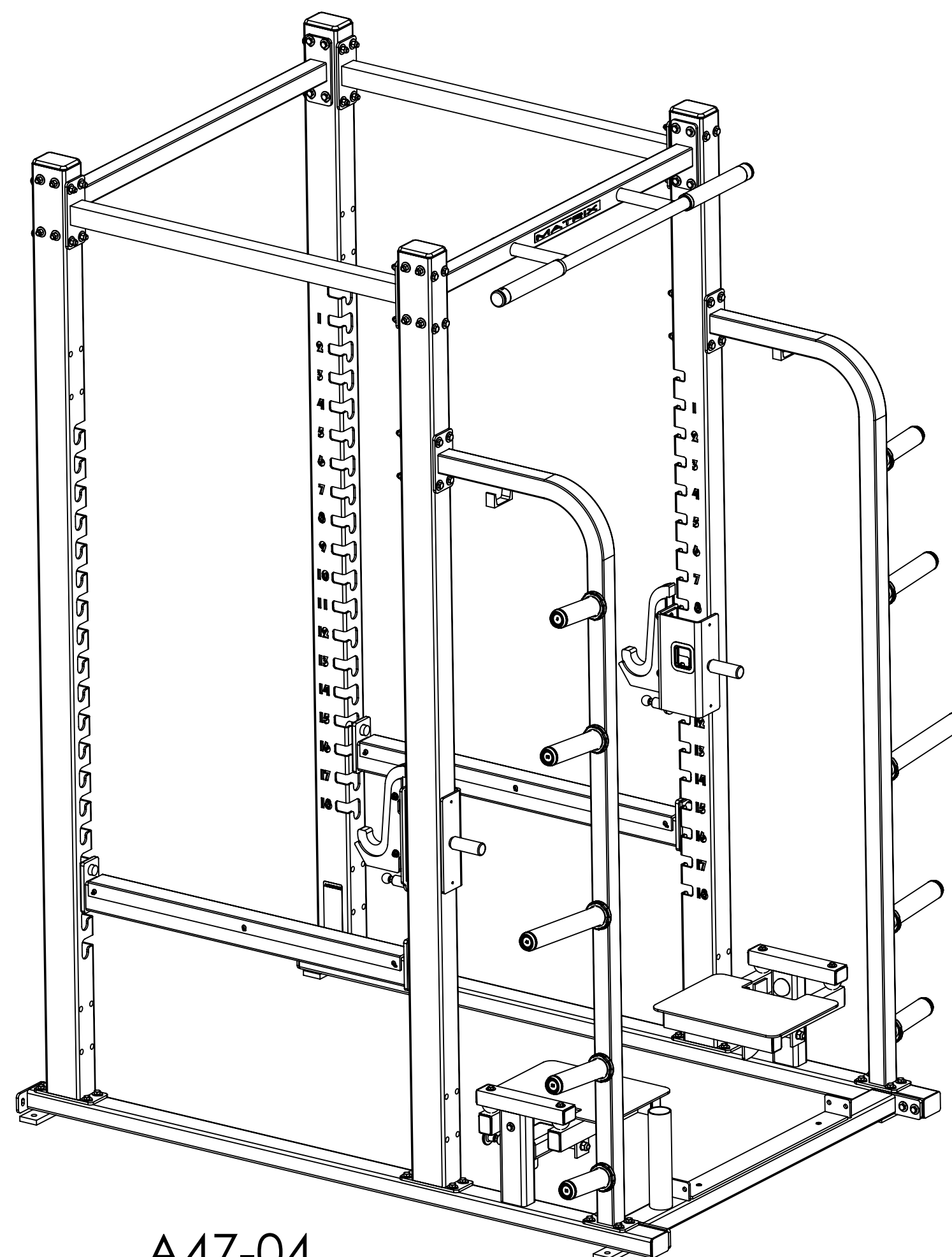
A47-04 (SHOWN IN EXPLODED VIEW SHEET 1)
