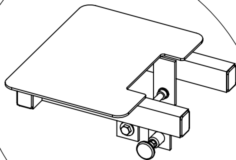
SPOTTER STAND RIGHT ORIENTATION (SHOWN EXPLODED)
