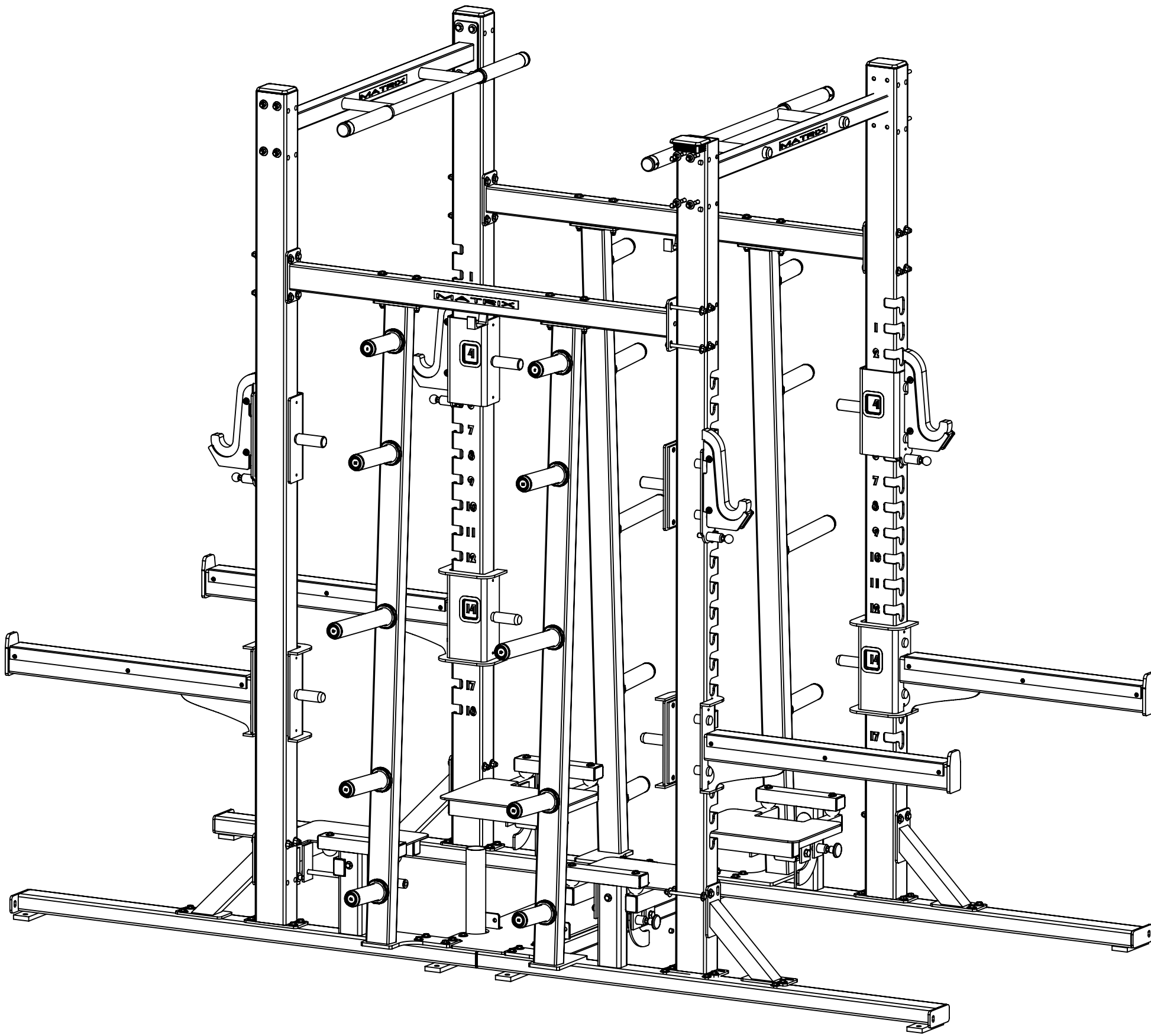
A691 M SHOWN IN EXPLODED VIEW SHEET 1
