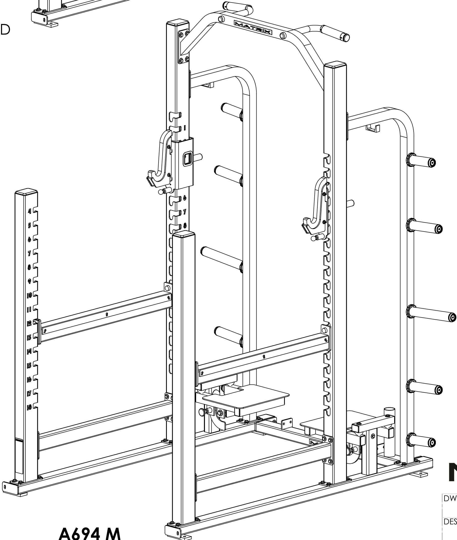
A694 M SEE SHEET 1 FOR EXPLODED VIEW
