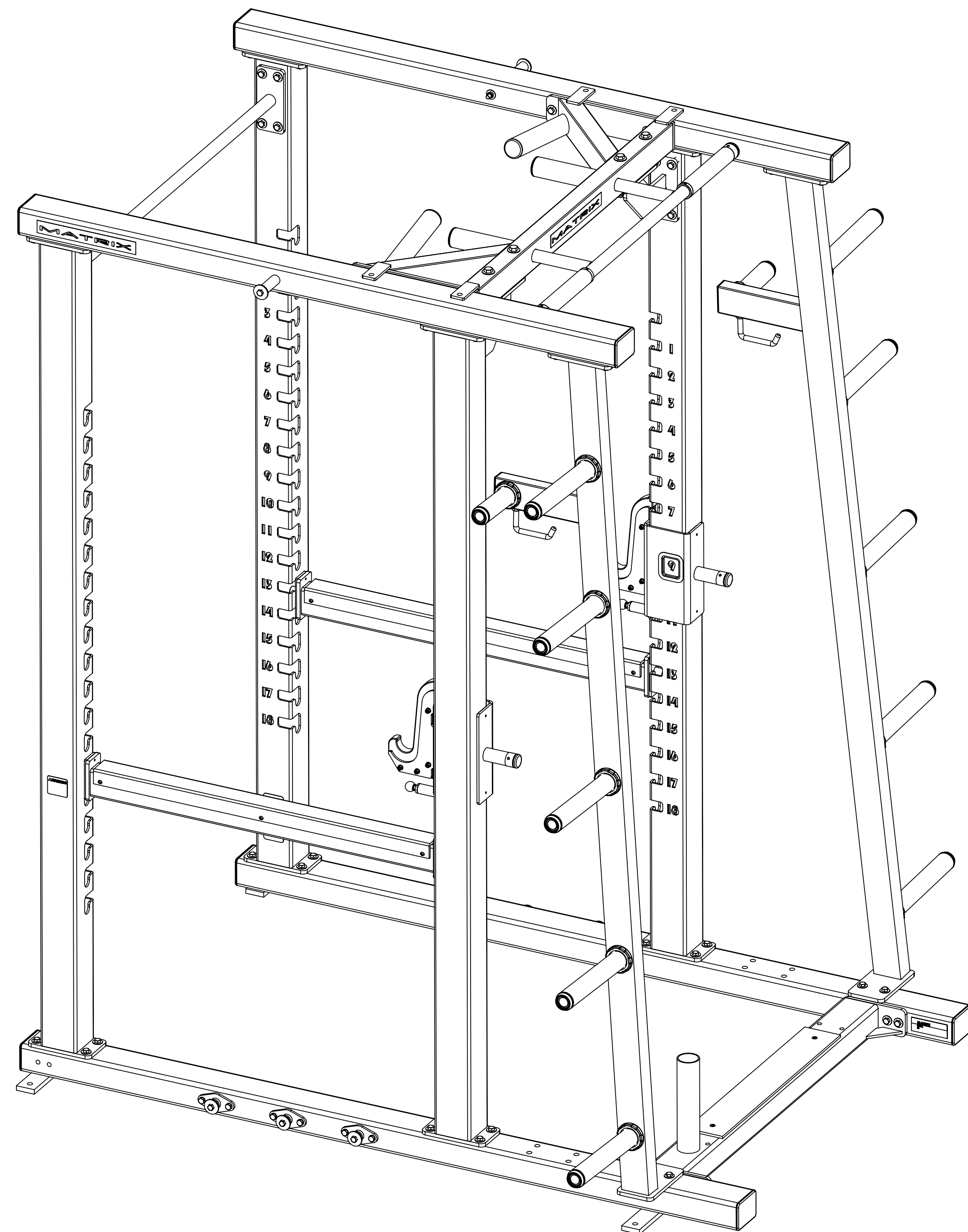
MR47-04 SHOWN IN EXPLODED VIEW SHEET 1
