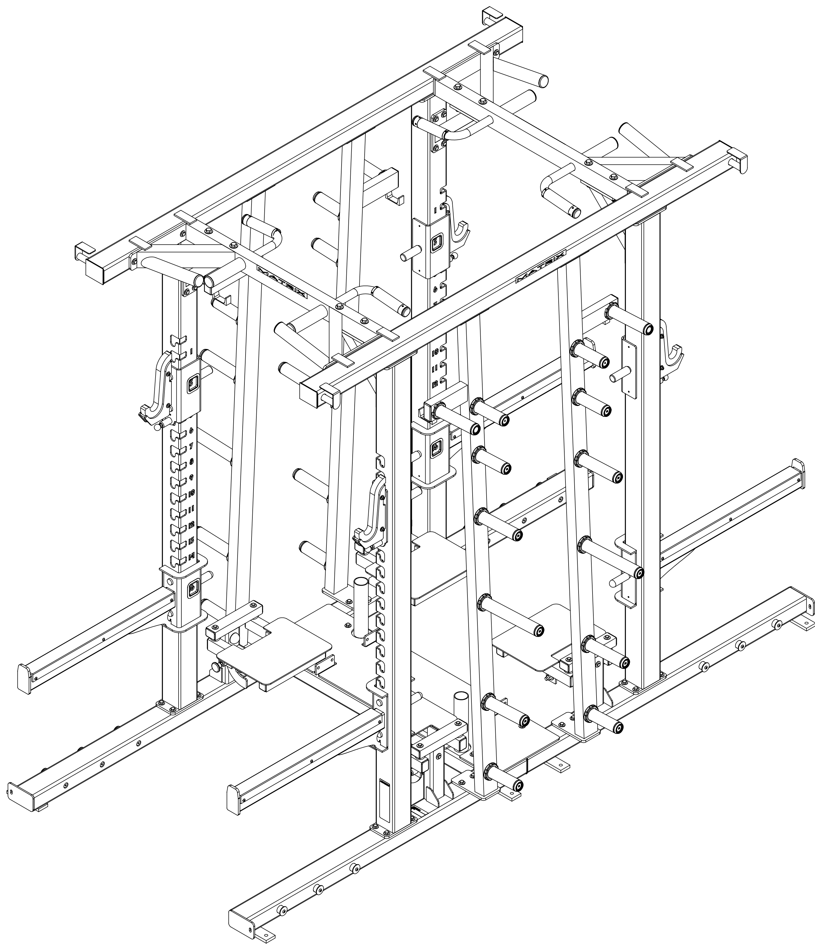
MR691 M SHOWN IN EXPLODED VIEW ON SHEET 1
