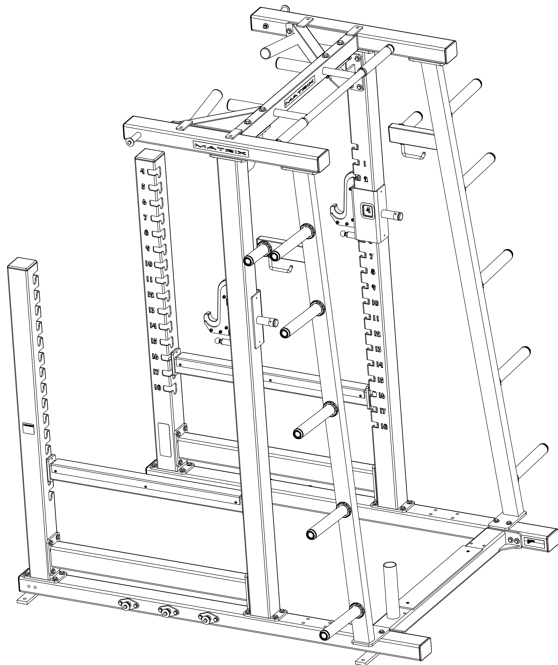
MR694-04 SHOWN IN EXPLODED VIEW SHEET 1
