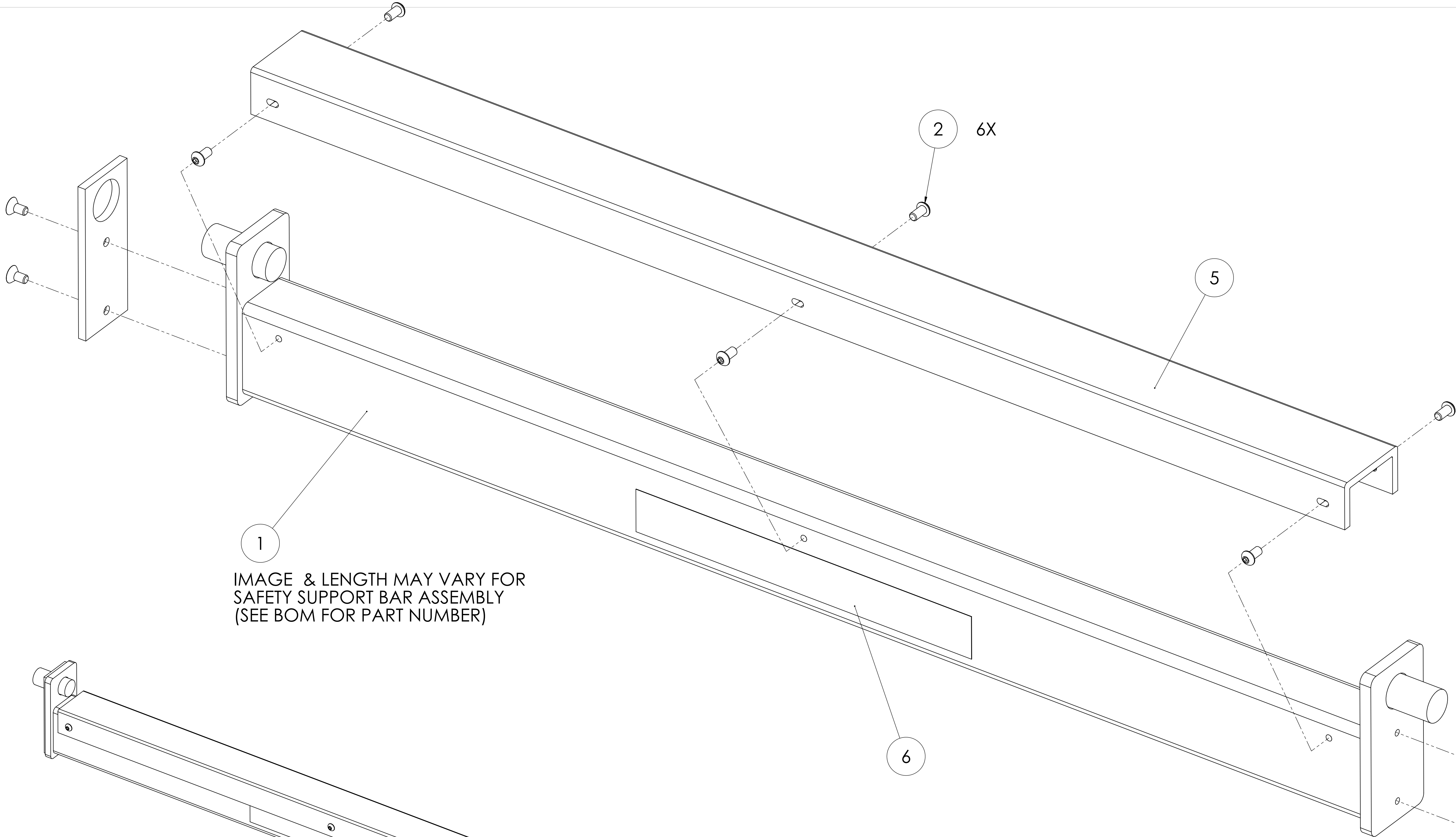
160-134 SAFETY SUPPORT BAR (SHOWN EXPLODED) (39.75 REF)
