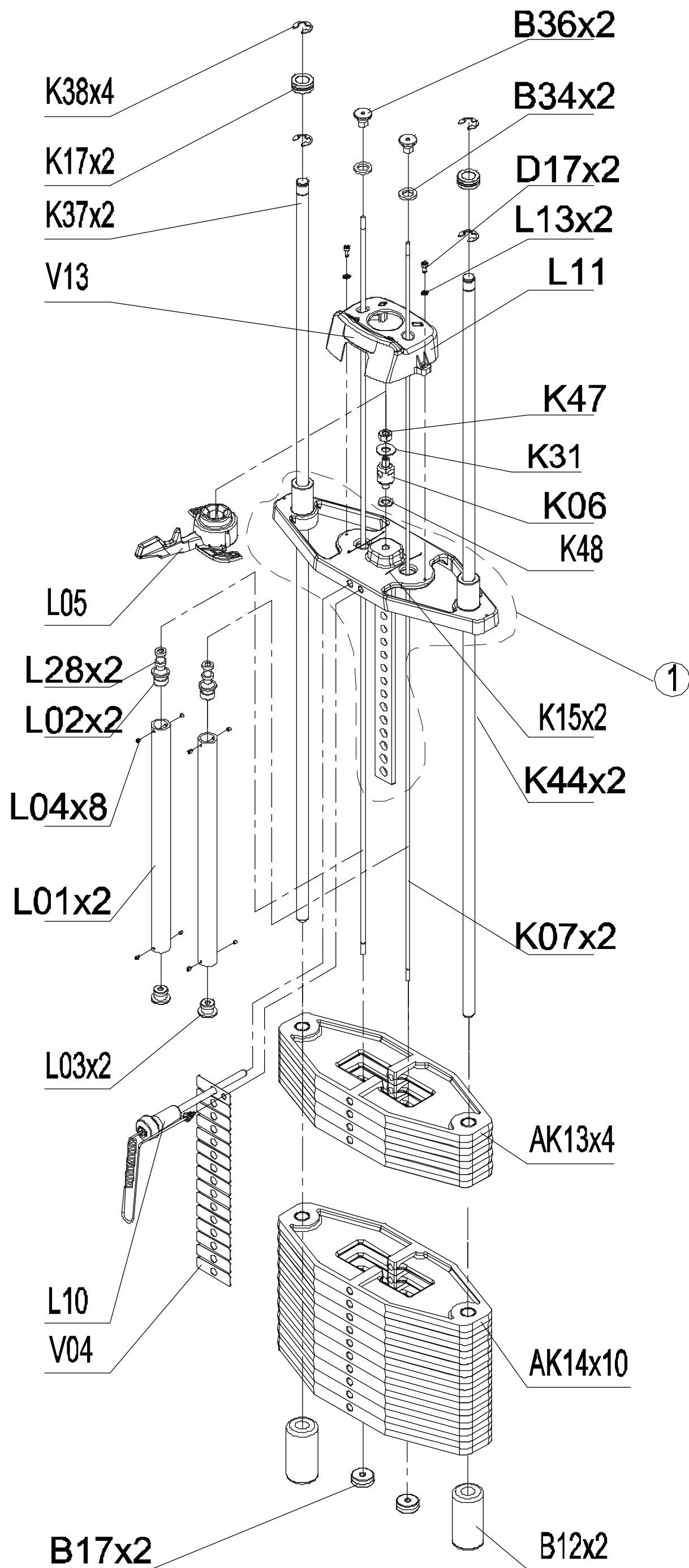
200LBS WEIGHT STACK SET
