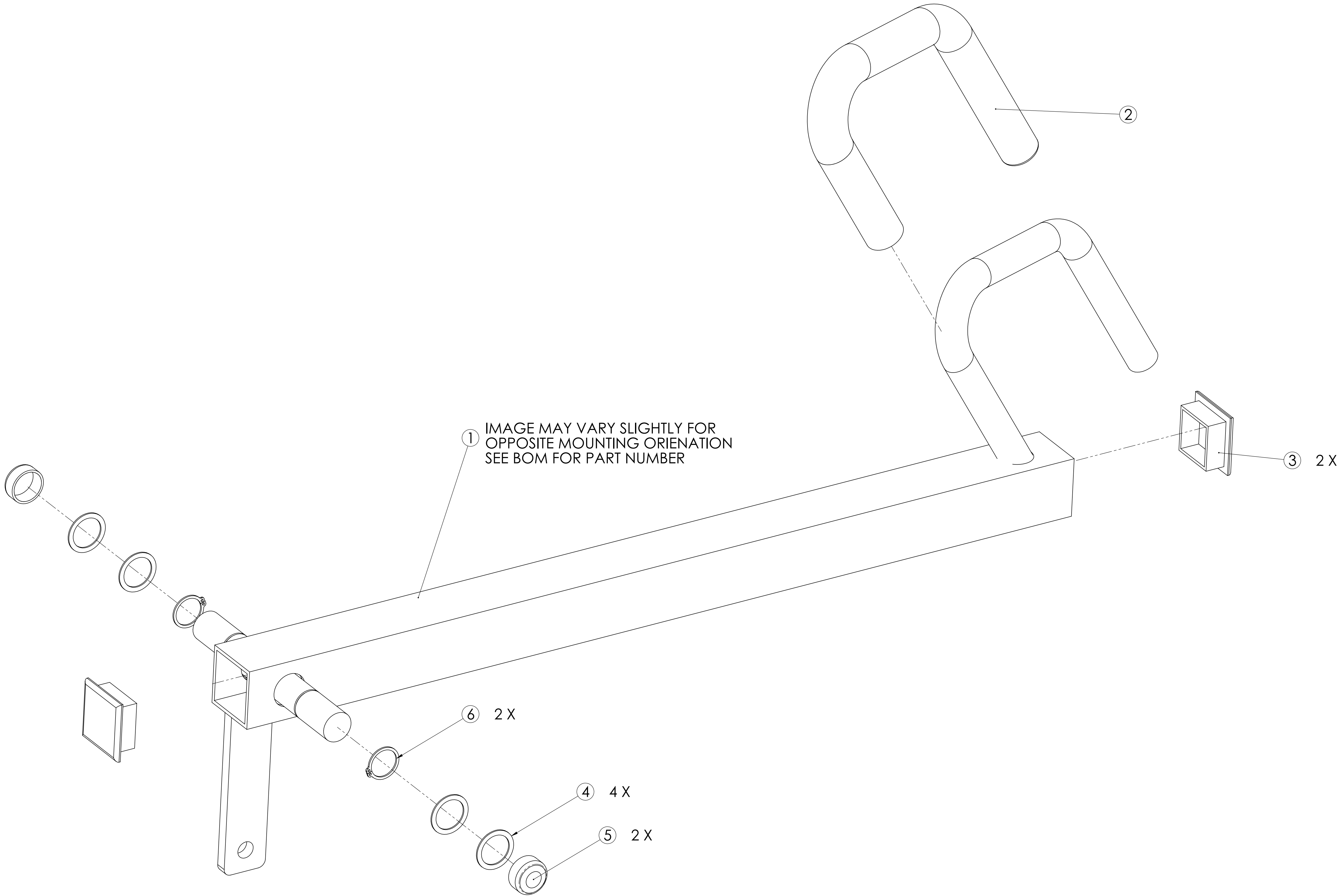
RIGHT HAND ARM ASSEMBLY (SHOWN EXPLODED)
