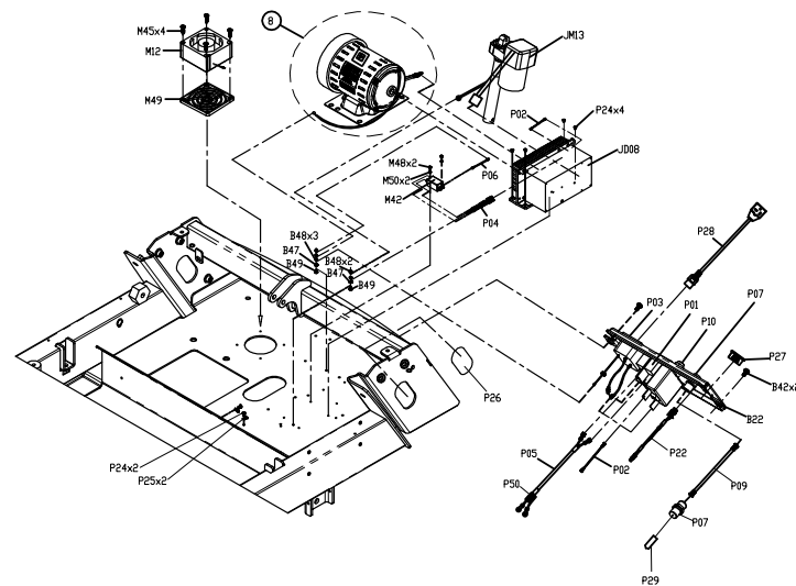
Detail View of Electrical Components
