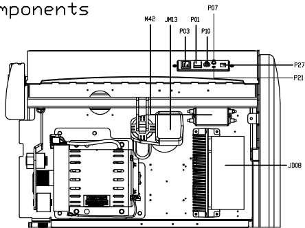
Top View of Electrical Components
