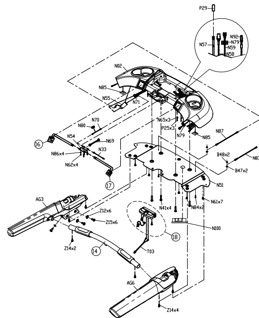
Detail view of Console Base
