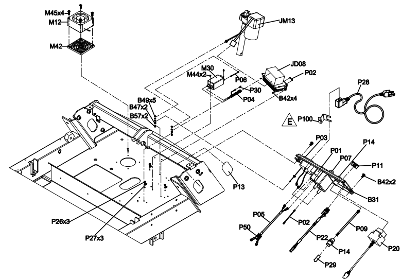
Detail View of Electrical Components
