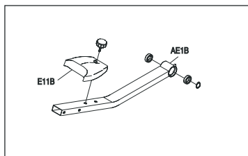
Threaded Toe Box Front Pedal Arm
