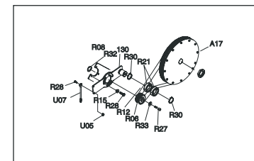
Timing Belt Crank Assembly
