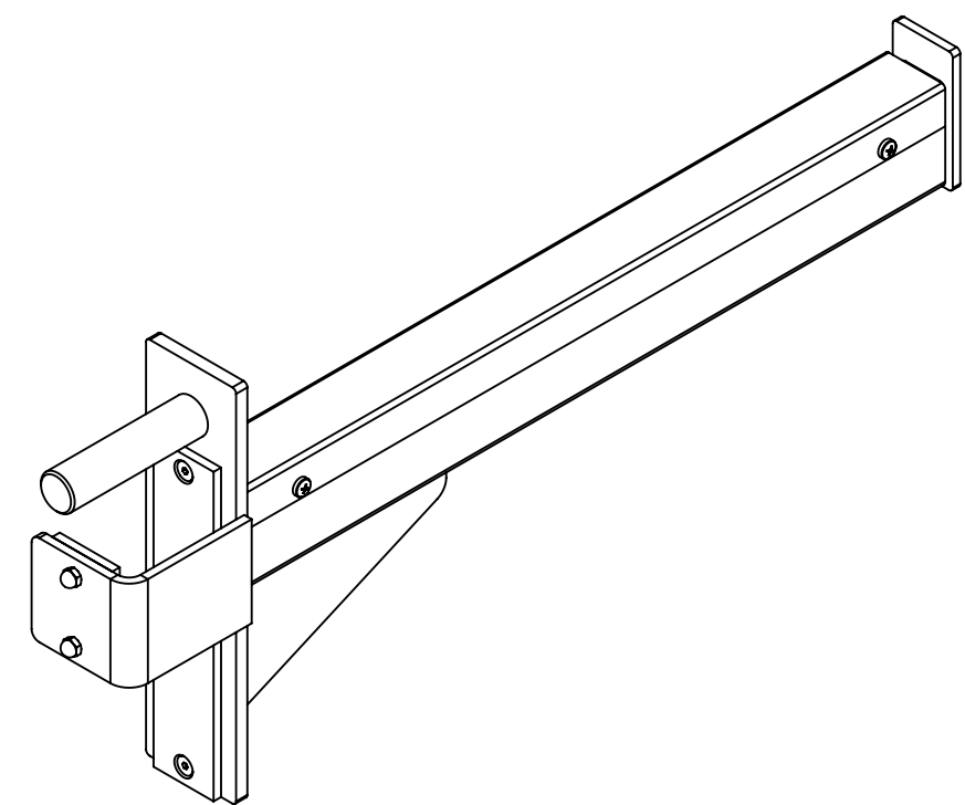
161-300 (SHOWN EXPLODED)
