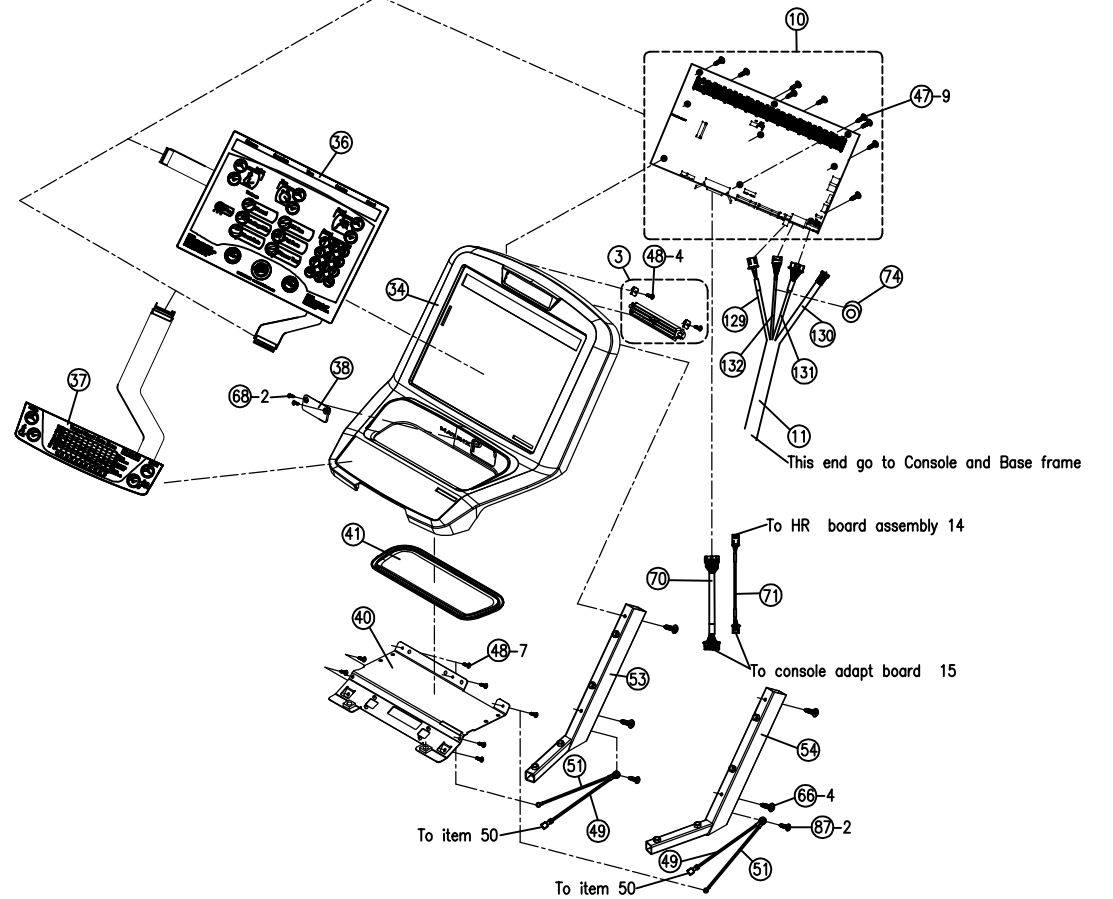
DETAIL VIEW OF FACE PLATE
