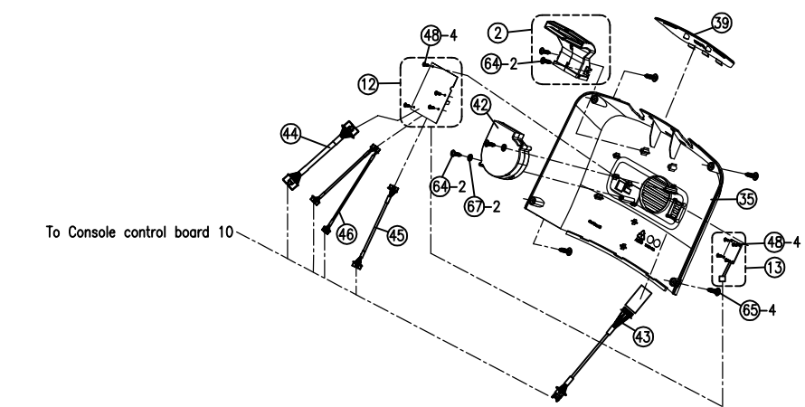
DETAIL VIEW OF BACK COVER
