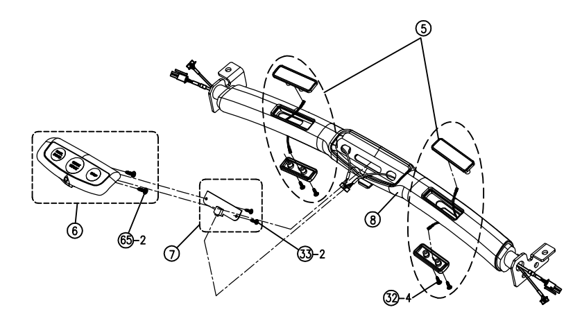
DETAIL VIEW OF CROSSBAR
