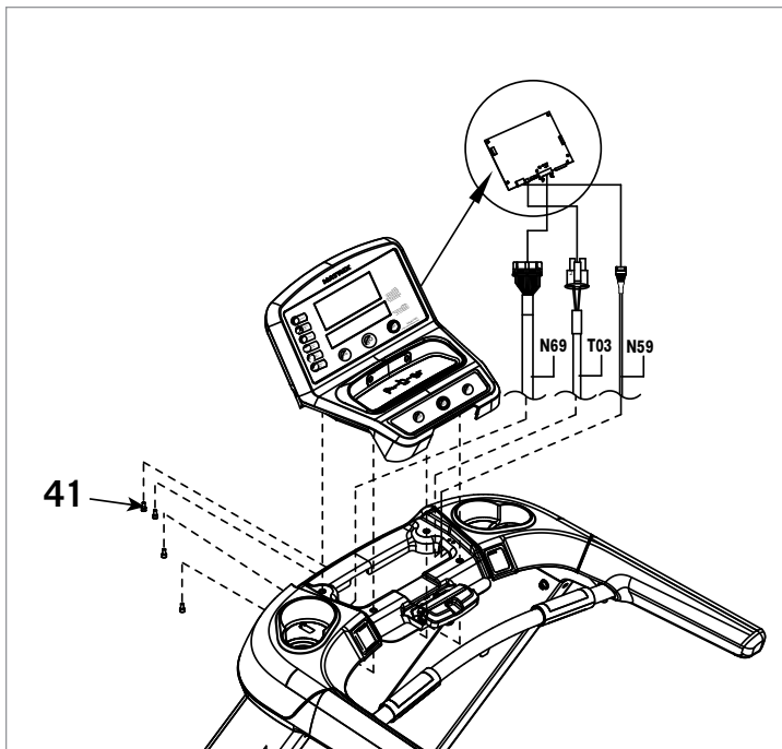
41 SOCKET HEAD CAP SCREW Qty: 4
