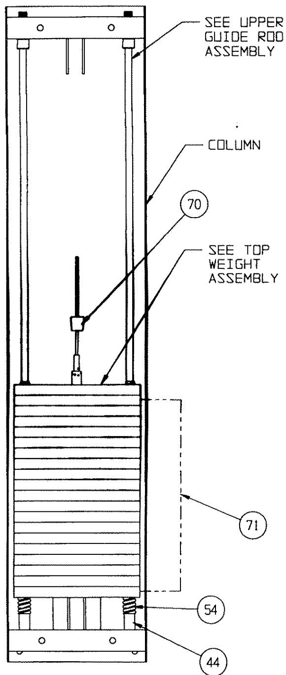
REAR VIEW
