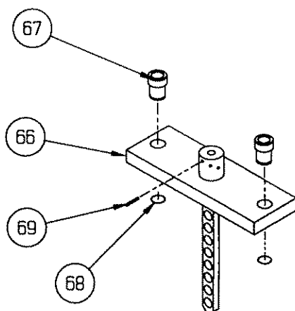
TOP WEIGHT ASSEMBLY
