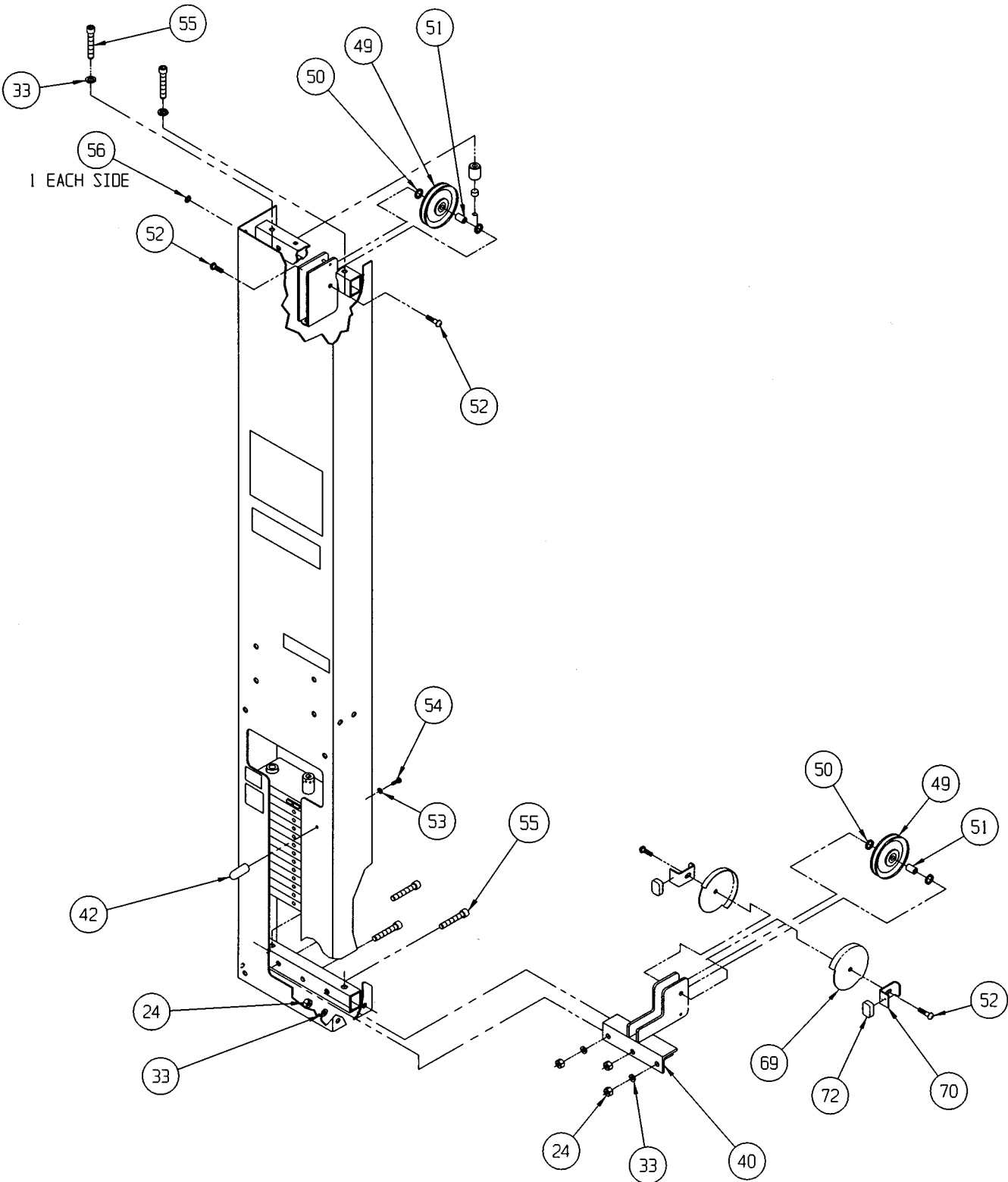
MODULAR CONFIGURATION
