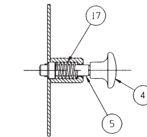
DETENT PIN DETAIL
