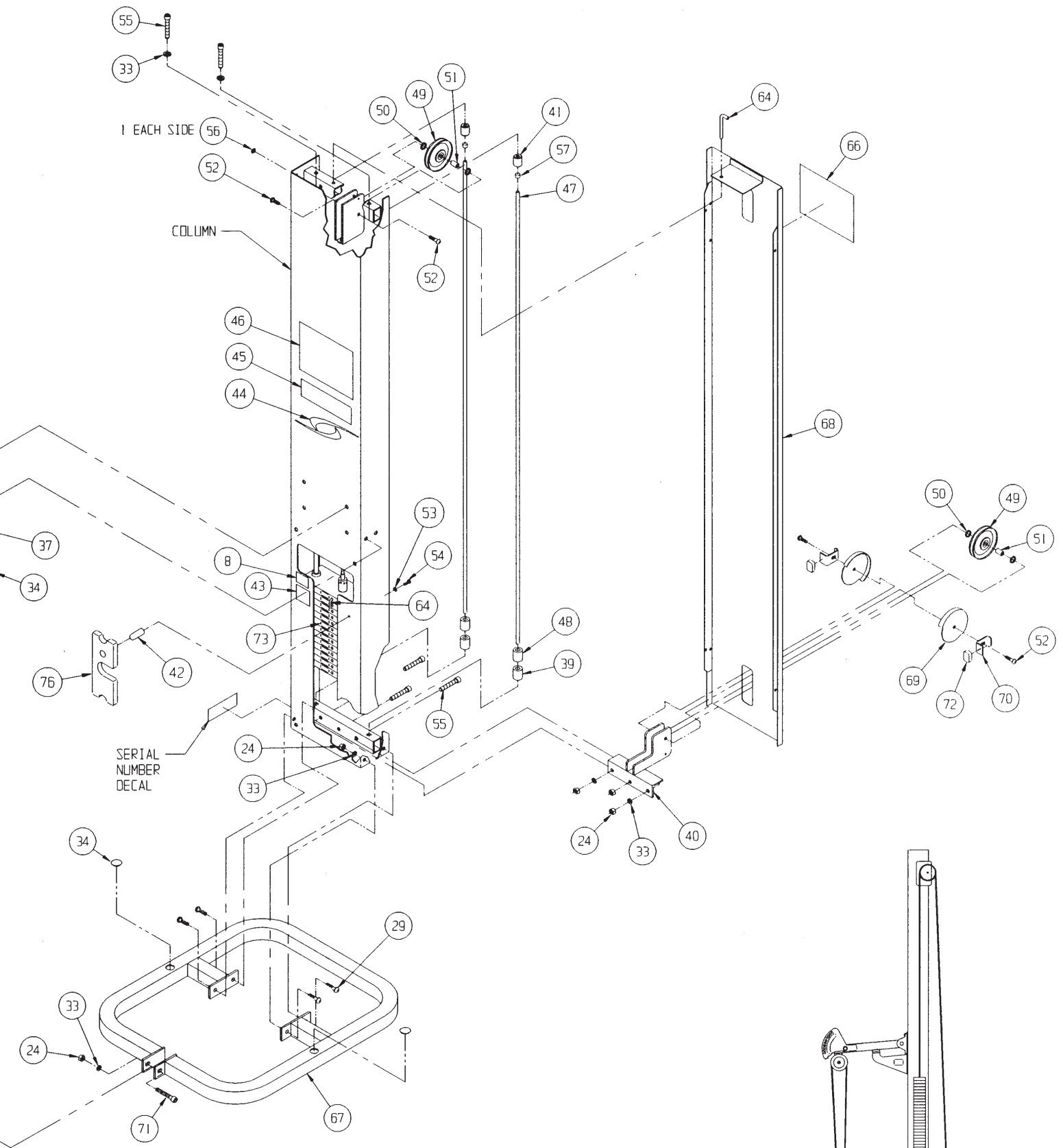
FREE STANDING CONFIGURATION
