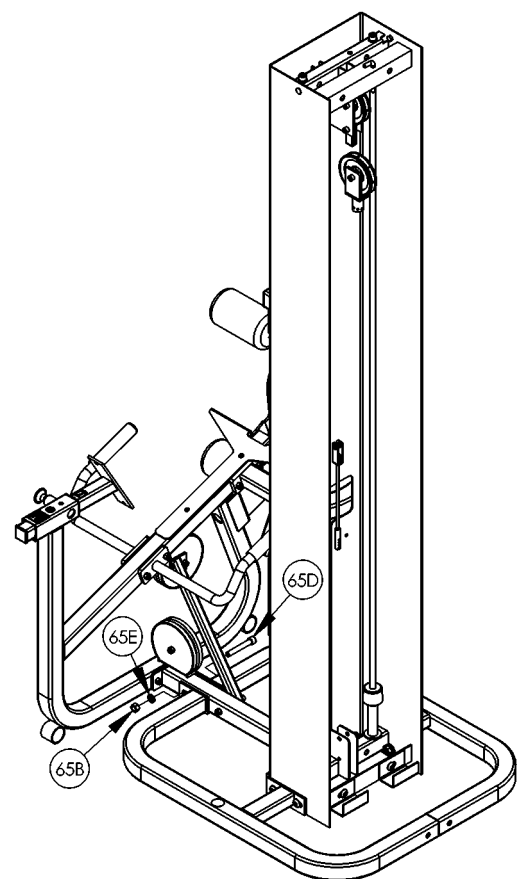
Cable Routing Detail
