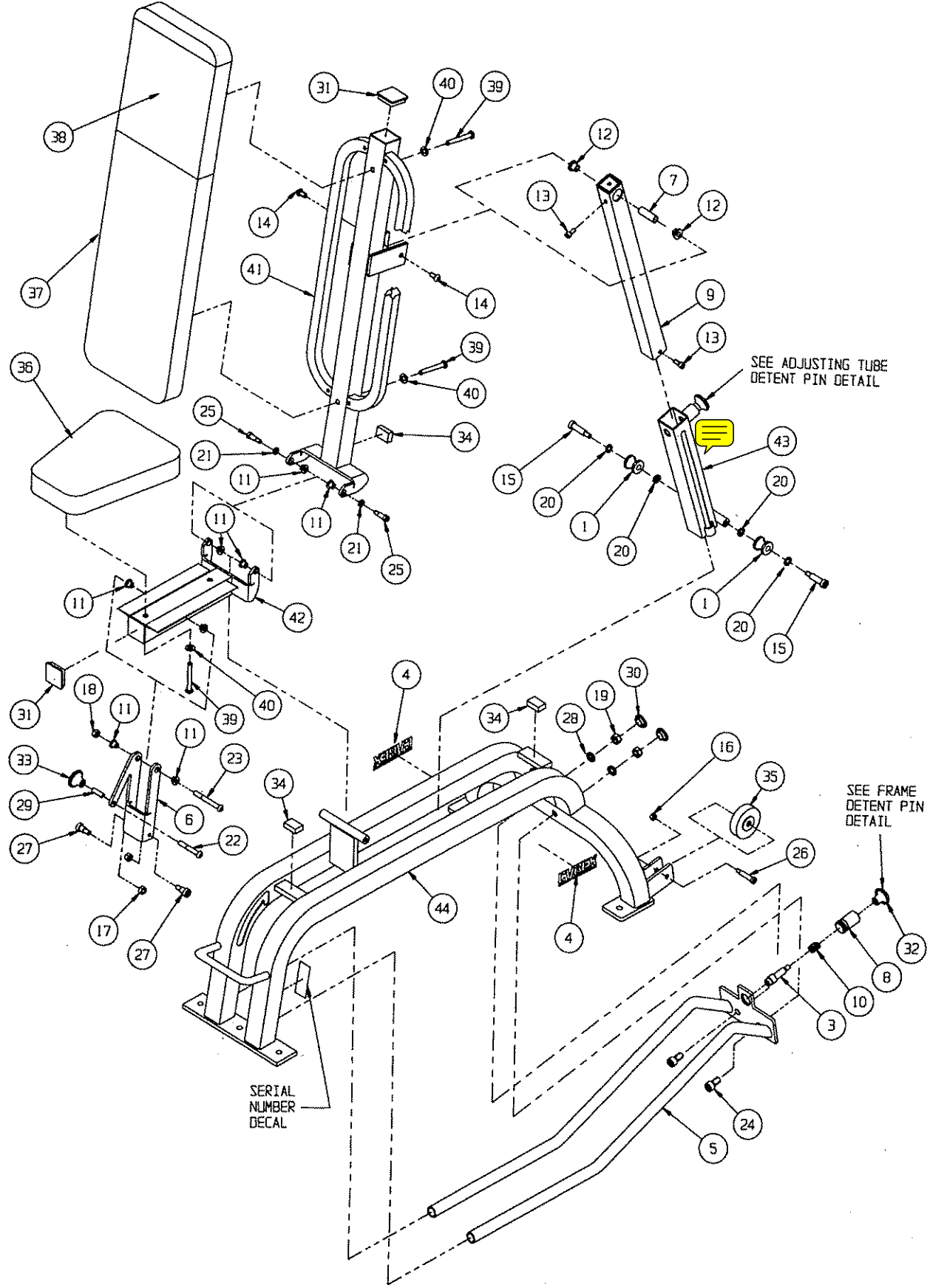
ADJUSTABLE FLAT TO 80 DEGREE BENCH (5435) EXPLODED-VIEW DIAGRAM
