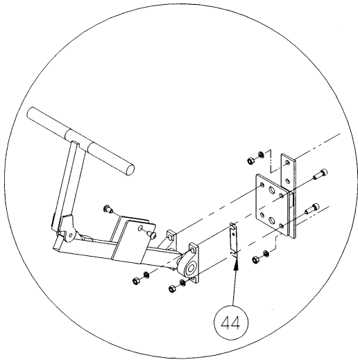
SHIM DETAIL
