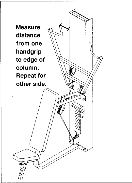
Figure 2 - Verifying Alignment
