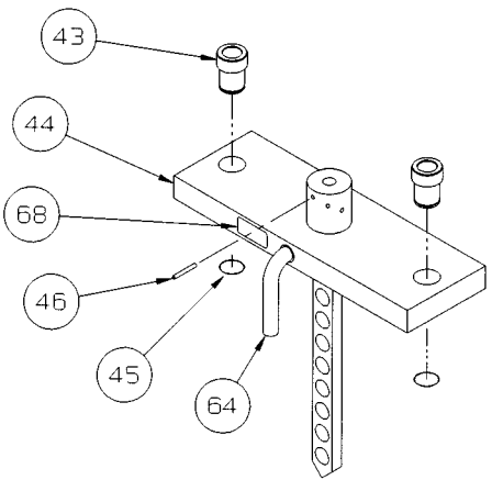
TOP WEIGHT ASSEMBLY
