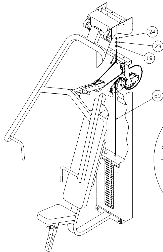
CABLE ROUTING DETAIL
