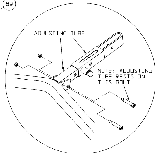
ADJUSTING TUBE ASSEMBLY DETAIL
