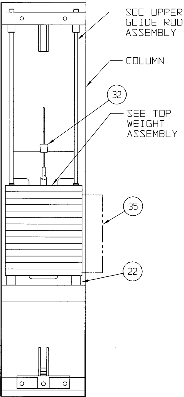
REAR VIEW
