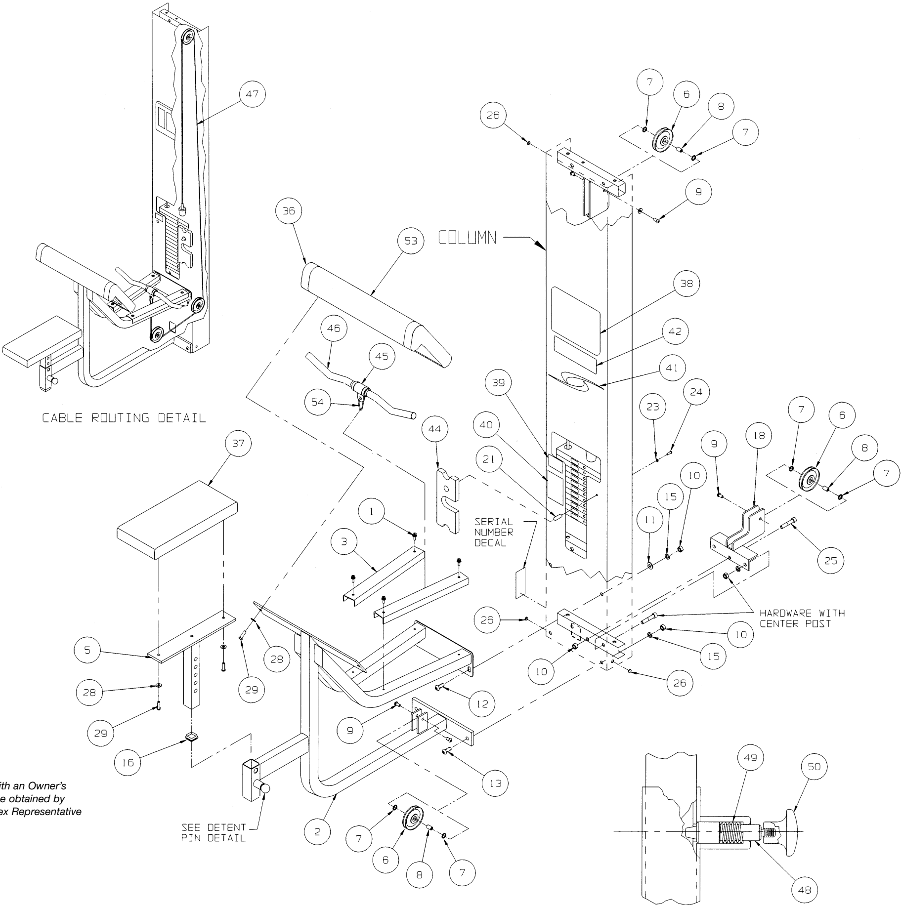
DETENT PIN DETAIL
