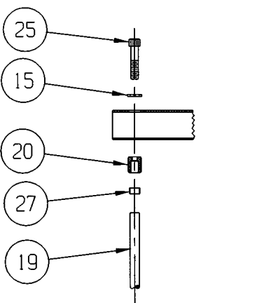
UPPER GUIDE ROD ASSEMBLY
