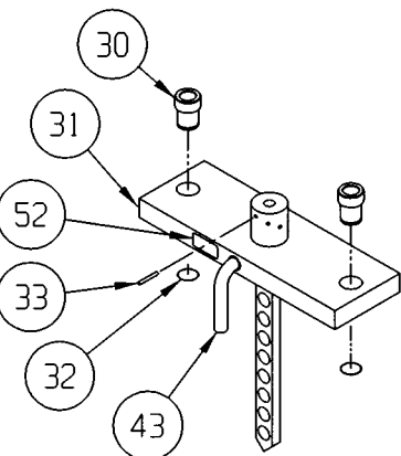
TOP WEIGHT ASSEMBLY
