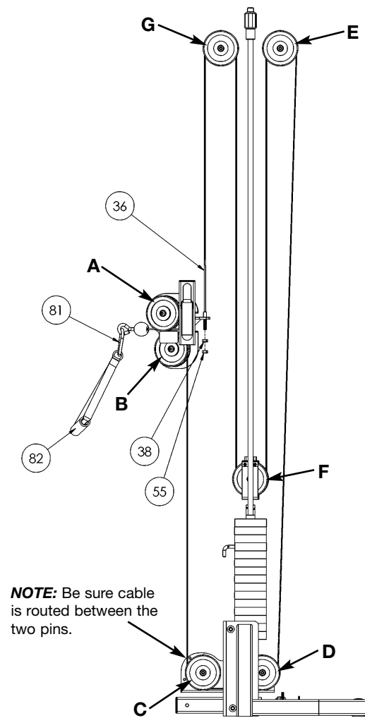
CABLE ROUTING DETAIL
