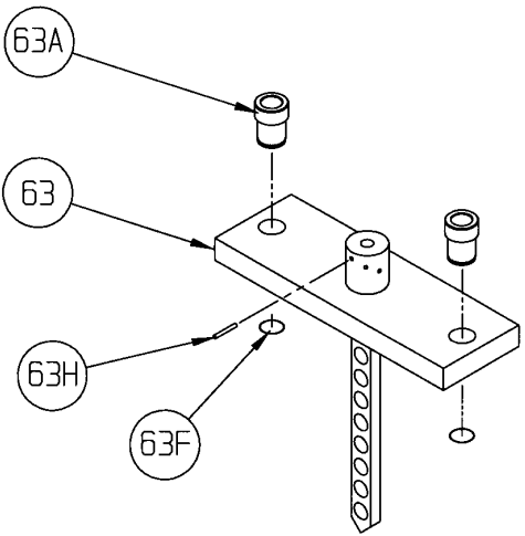
TOP WEIGHT ASSEMBLY
