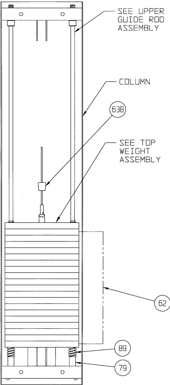
REAR VIEW
