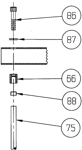
UPPER GUIDE ROD ASSEMBLY
