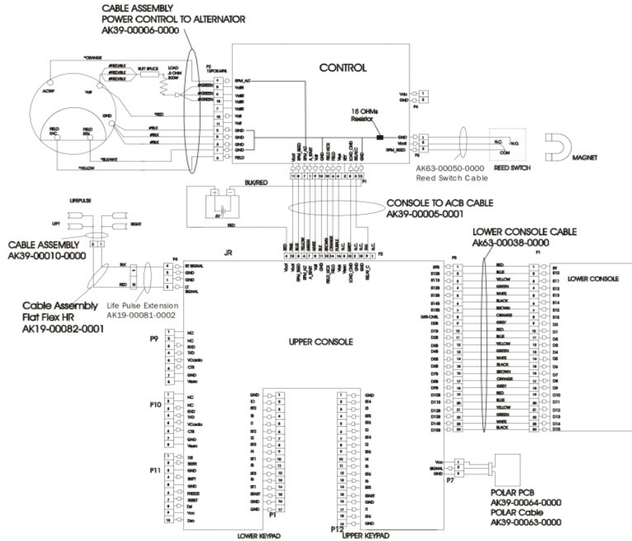
Cable Coax - AK32-00020-0001 Cable Power Ext - AK32-00078-0001
