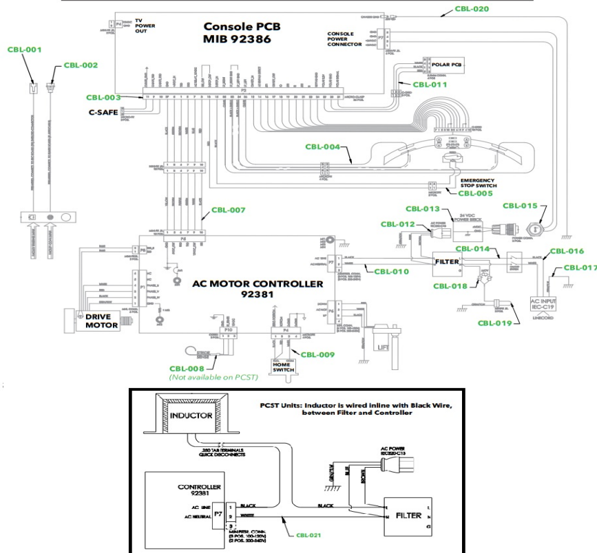
Electric Wiring Diagrams and Cable Parts List - DISCOVER
