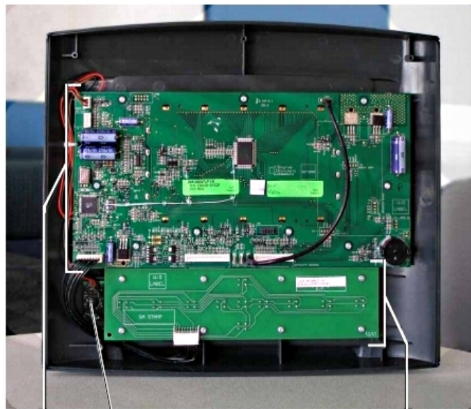
Telemetry PCB 8046001 Main Console PCB 8043501
