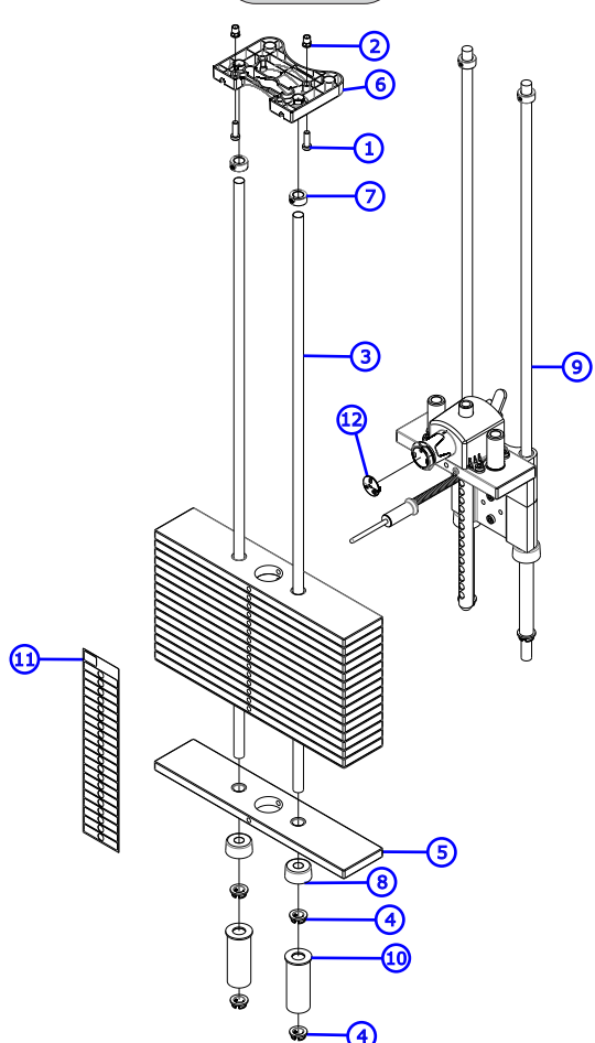
Uses 9423912 Cable (81.625")
