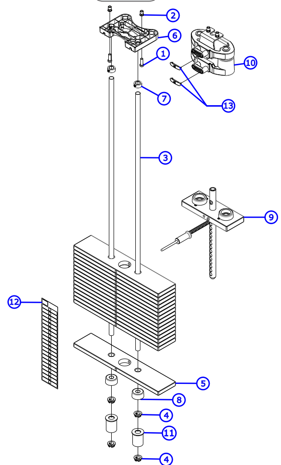
Uses 9423911 Cable (83.875")
