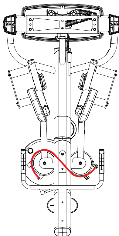
Figure 8 Cable (BOTTOM)
