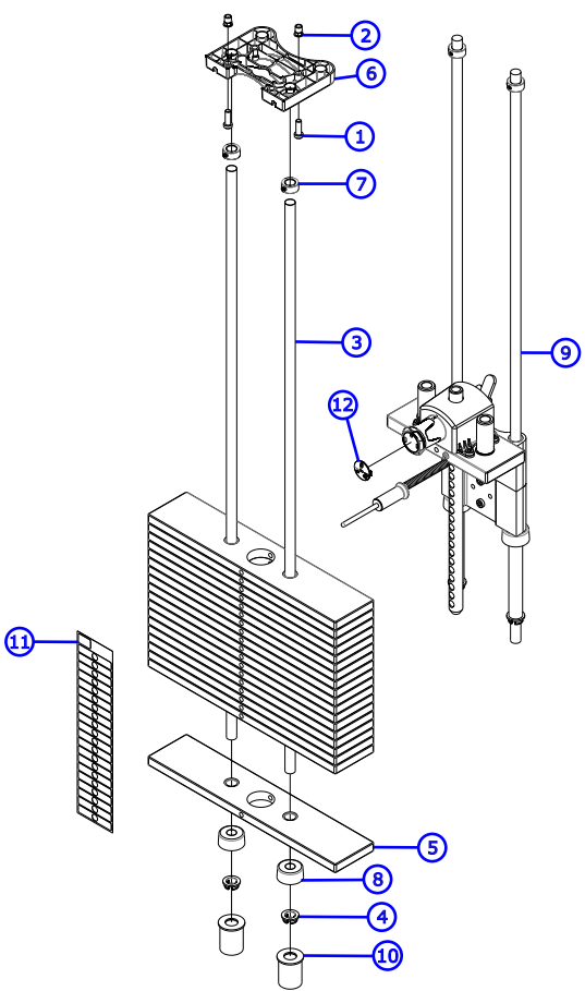
Uses 923914 Cable (110.188")
