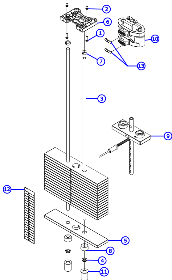
Uses 9423913 Cable (112.438")
