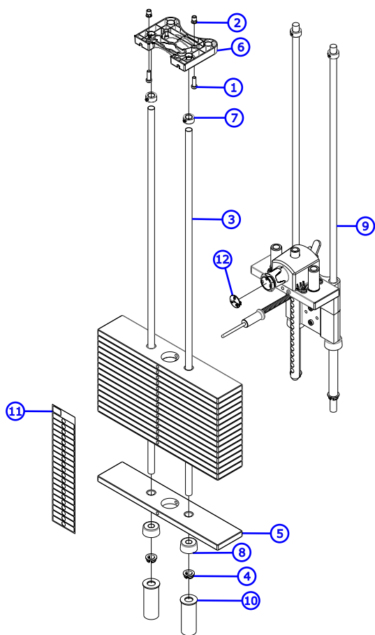
Uses 9423914 Cable (110.188")
