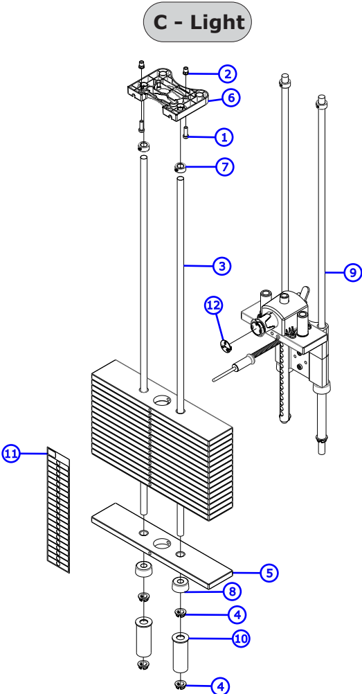
Uses 9424804 Cable (224")
