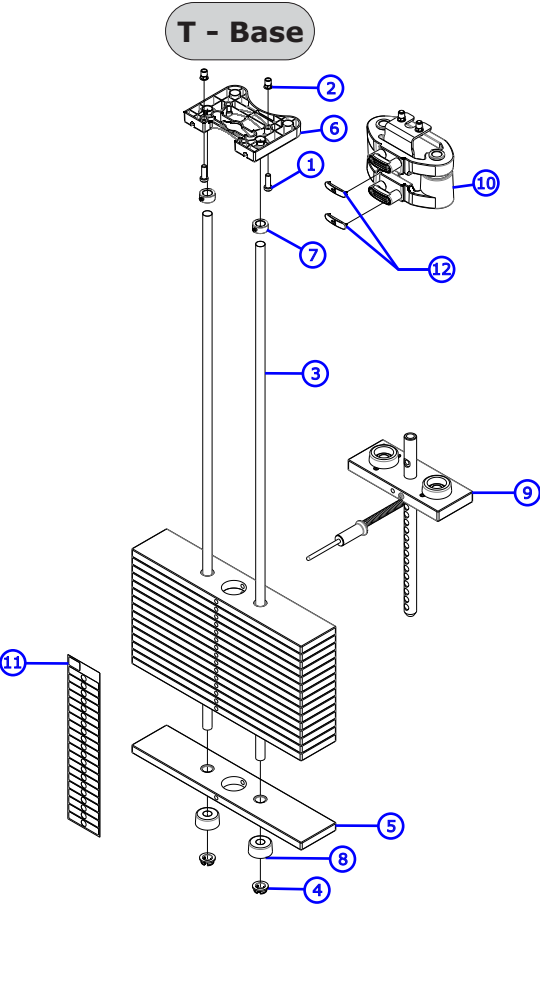
Uses 9424809 Cable (235.5")
