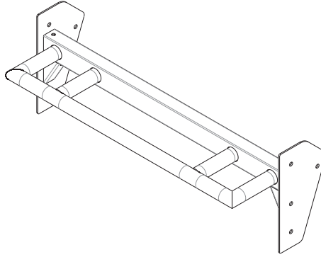
9042700 LARGE EXT
