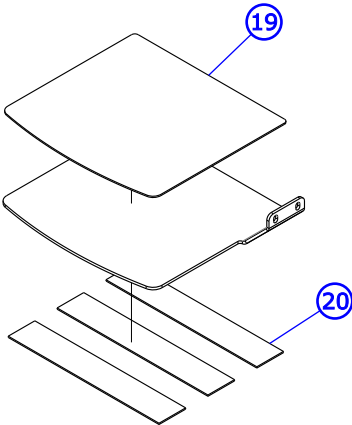
FOOTPLATE
