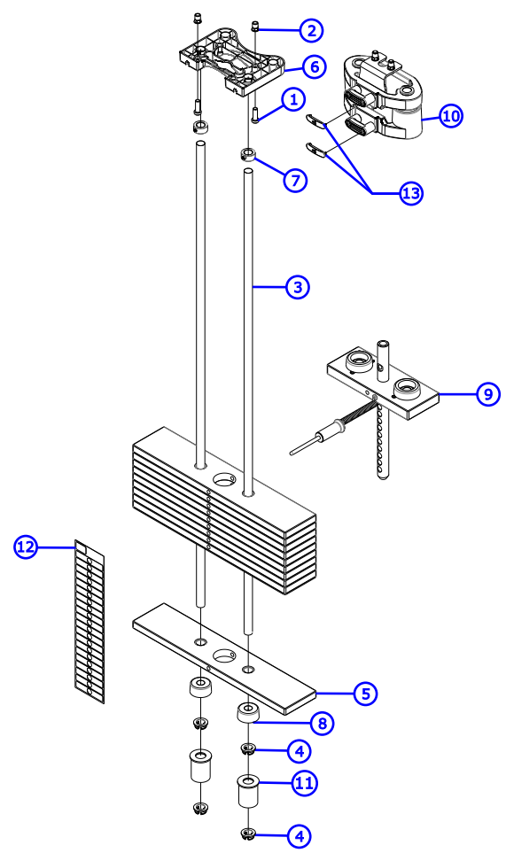
Uses 9423919 Cable (140.25")
